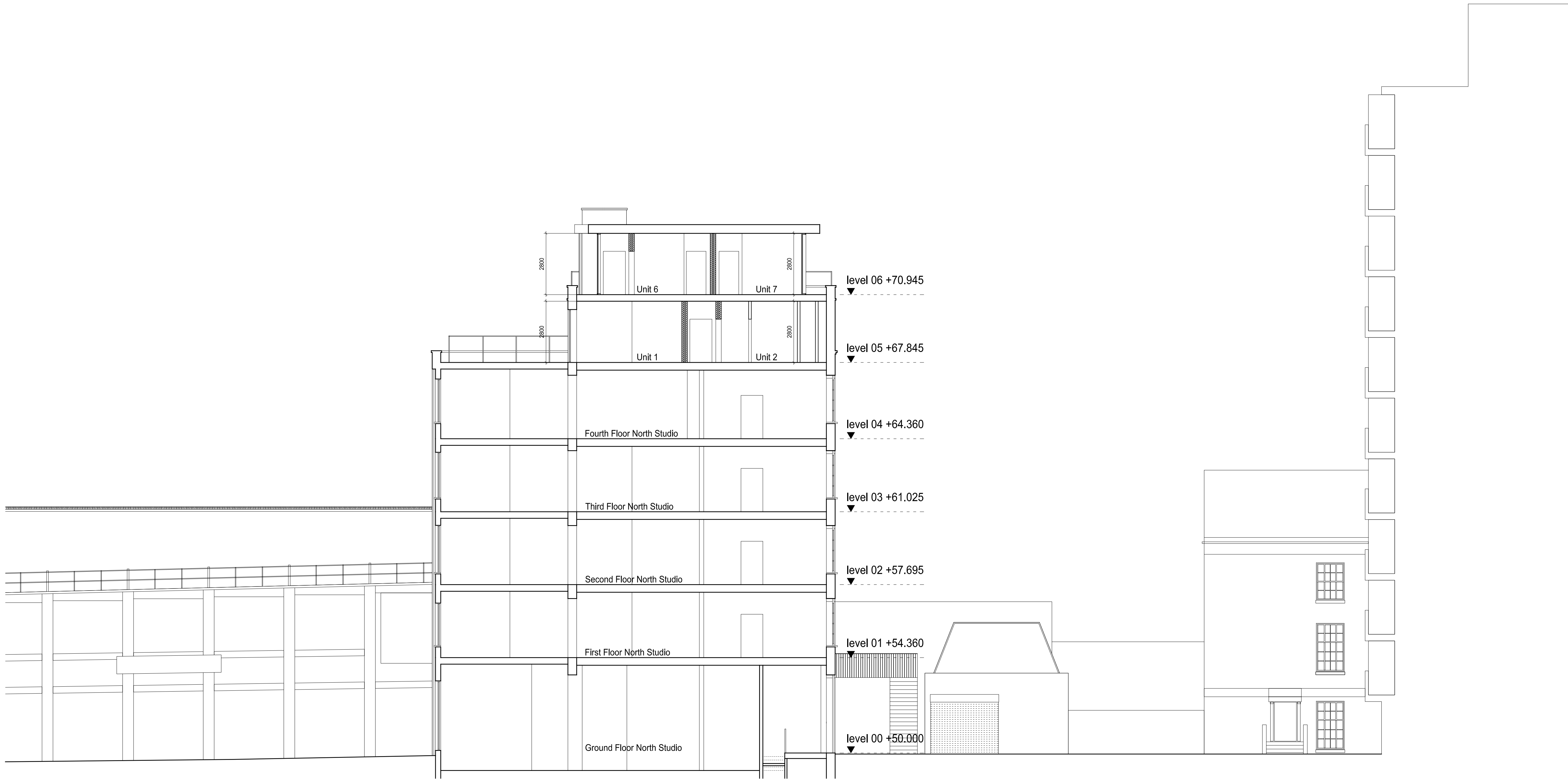
EXISTING D-D' SECTION
