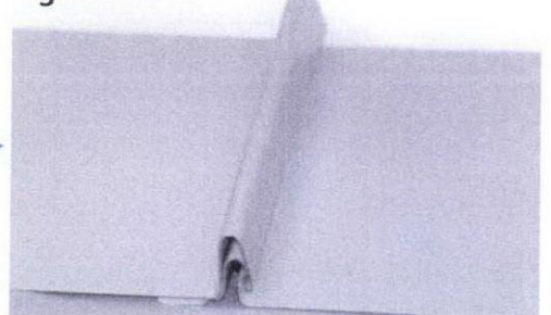
25mm high Urban Seam® Profile, with integrated eyelet hole fixing strip
