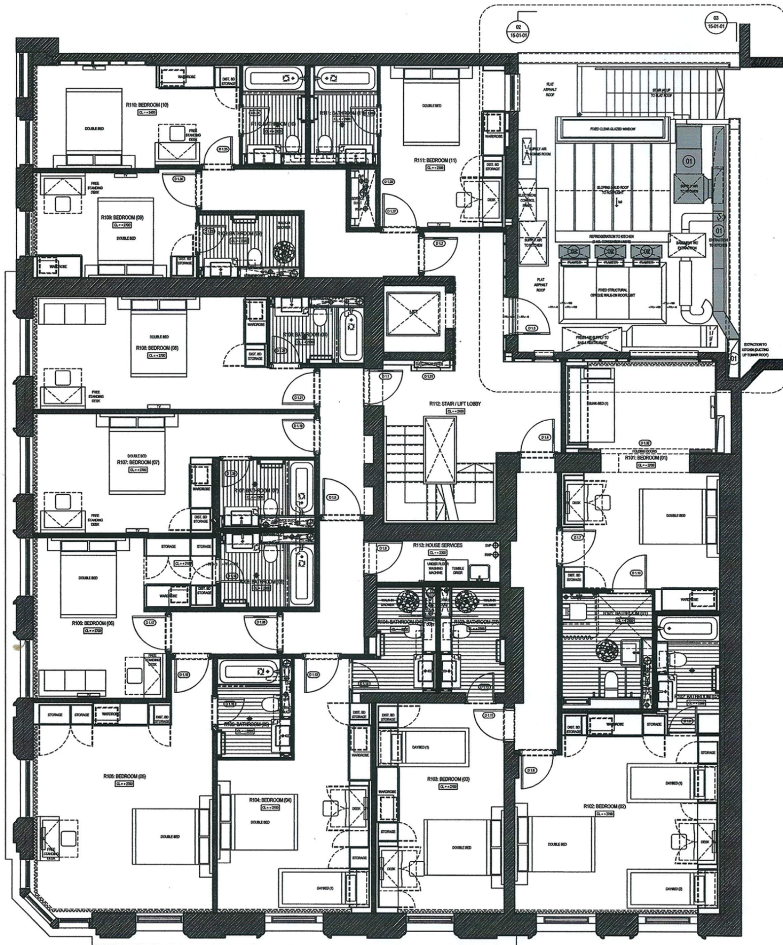
01 FIRST FLOOR: GENERAL ARRANGEMENT PLAN 01 (SHOWING PLANT EQUIPMENT LOCATION TO FLAT ROOF) Scale 1:50 (@A1 SIZE)
