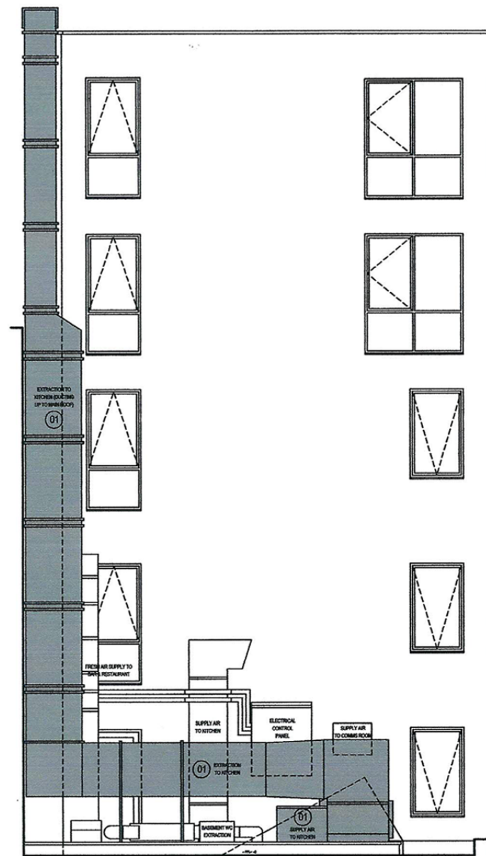
03 SIDE ELEVATION 03 (15-01-02) Scale 1:50 (@A1 SIZE)
