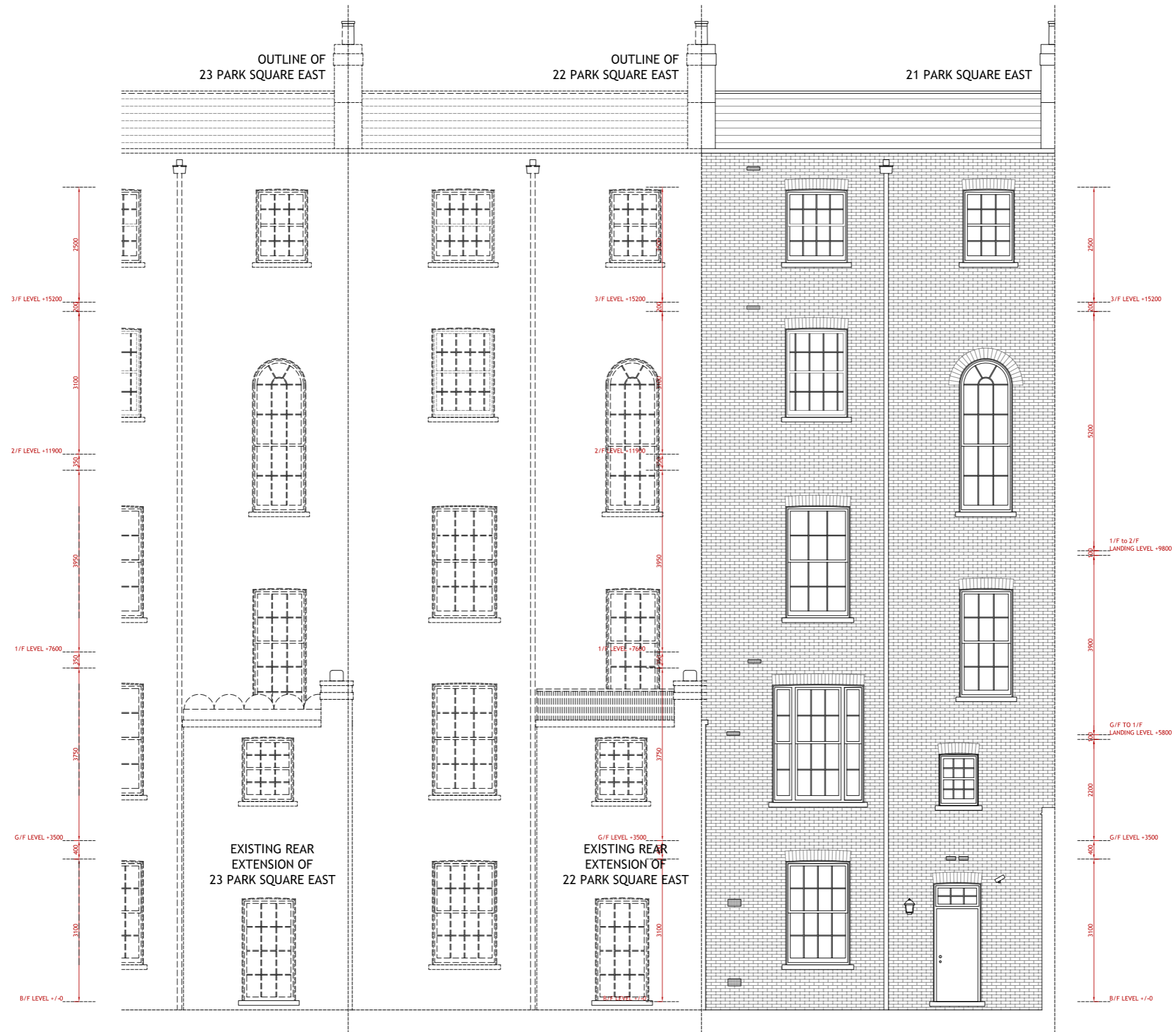
REAR ELEVATION AS EXISTING
