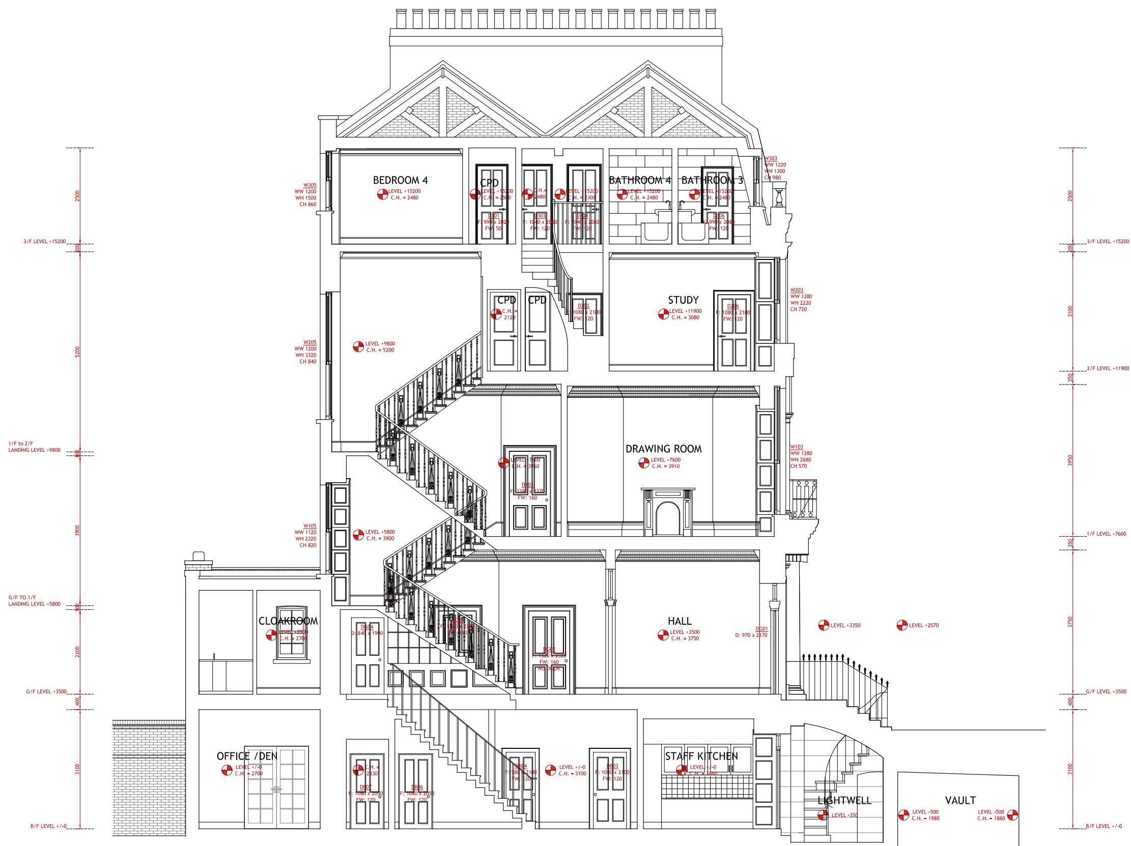
SECTION AA AS PROPOSED
