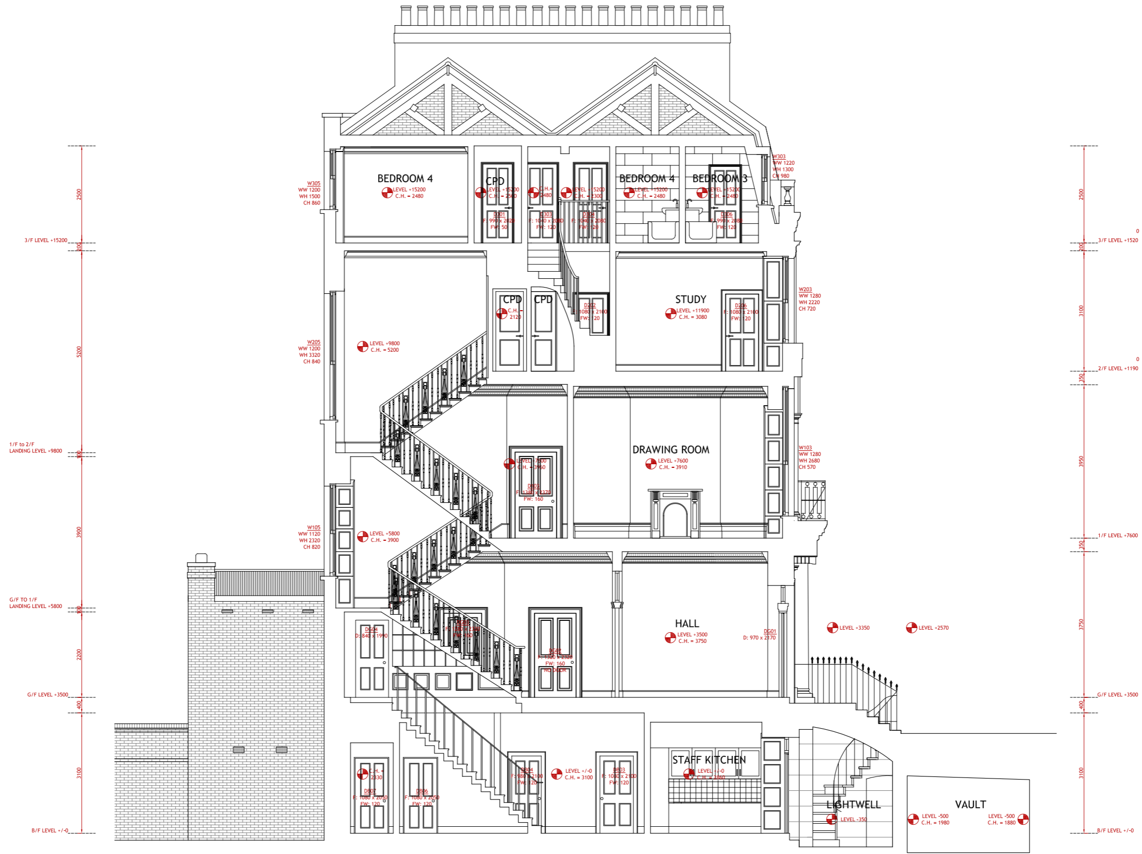
SECTION AA AS EXISTING
