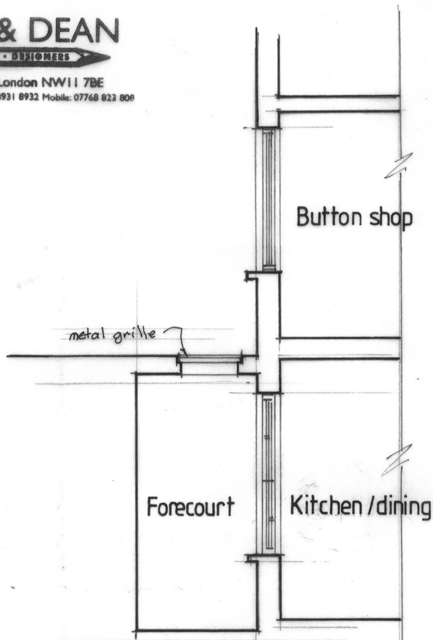
SECTION G-G
