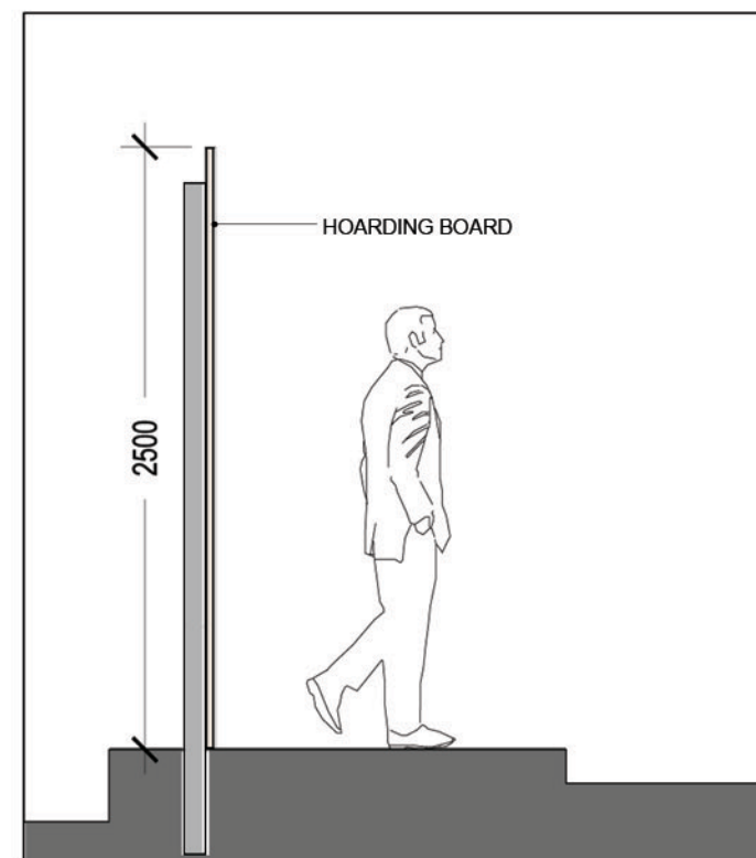
HOARDING BOARD TYPICAL CROSS SECTION
