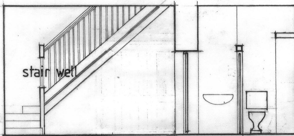
PROPOSED SECTION E-E
