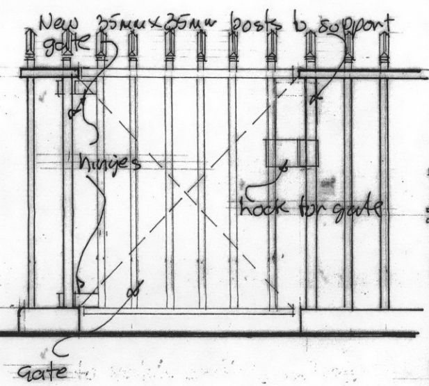
Gate detail
