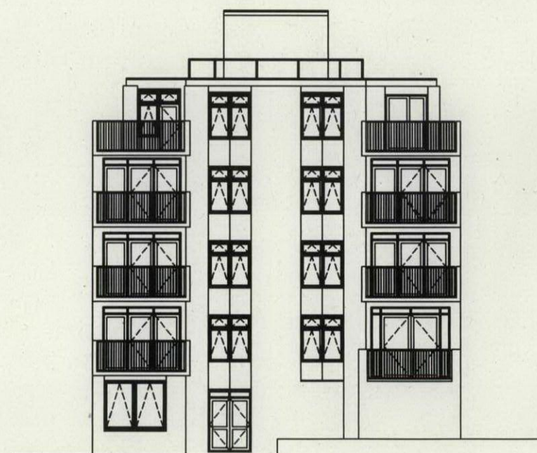
Rear Elevation (Garden)
