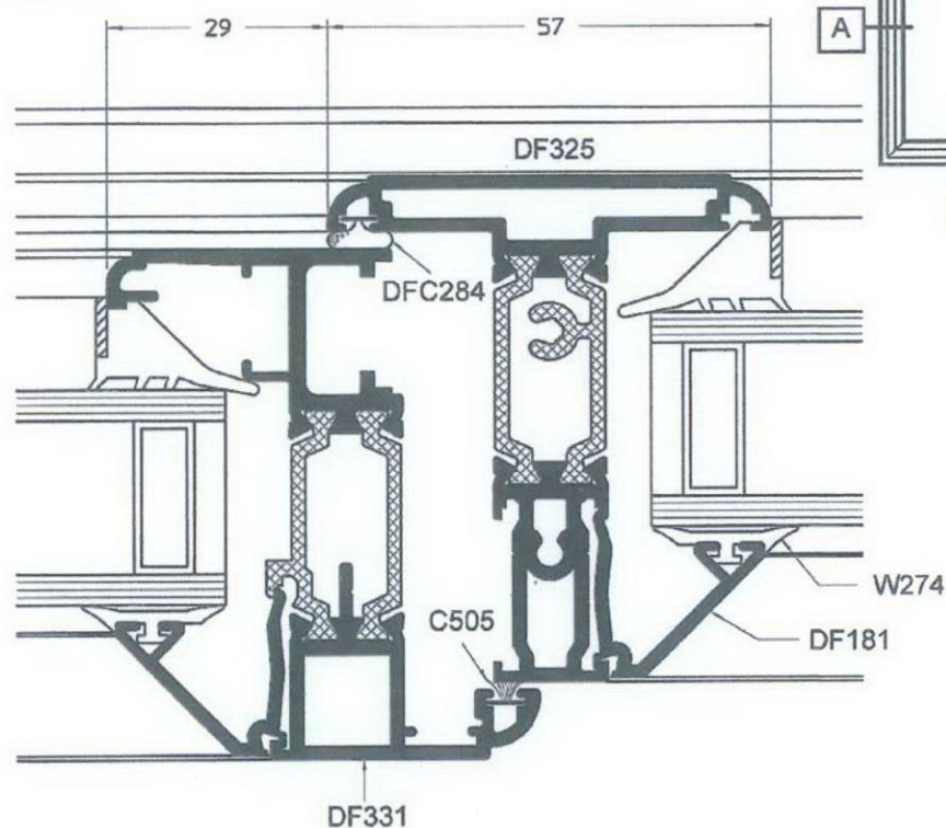
B Mullion / Vent
