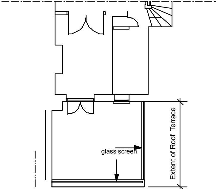
PROPOSED PART FIRST FLOOR PLAN and ROOF TERRACE PLAN
