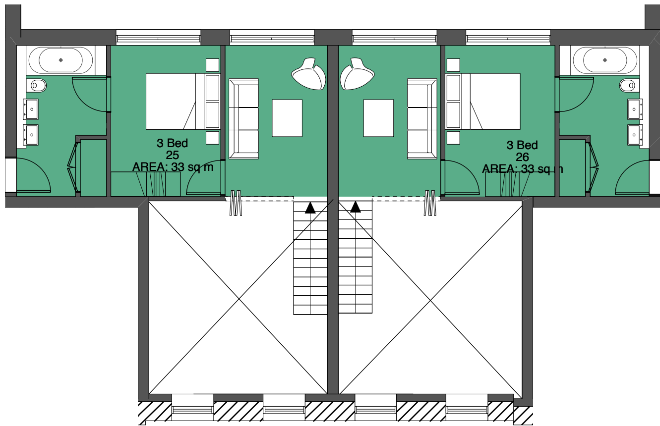
duplex apartments 25 & 26 Third Floor Plan - alternative 3 bedroom, 5 person layouts
