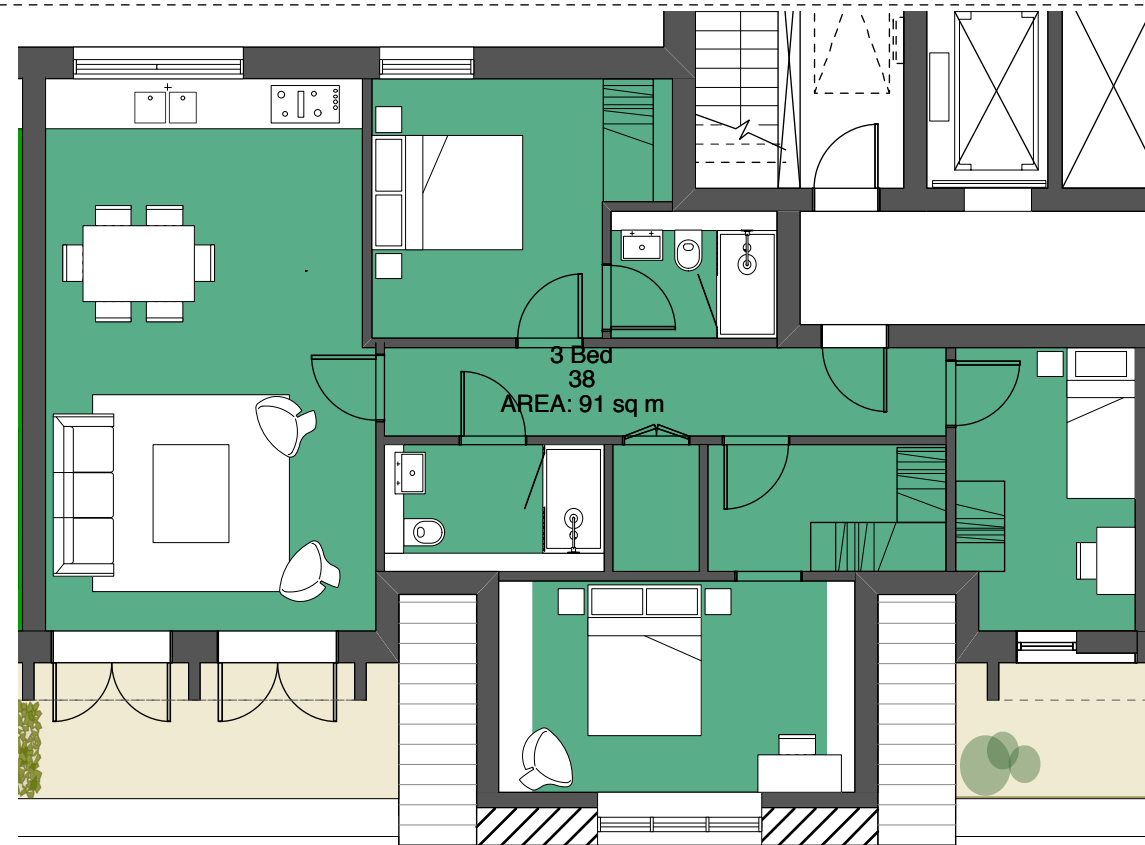
apartment 38 Fourth Floor Plan - alternative 3 bedroom, 5 person layout
