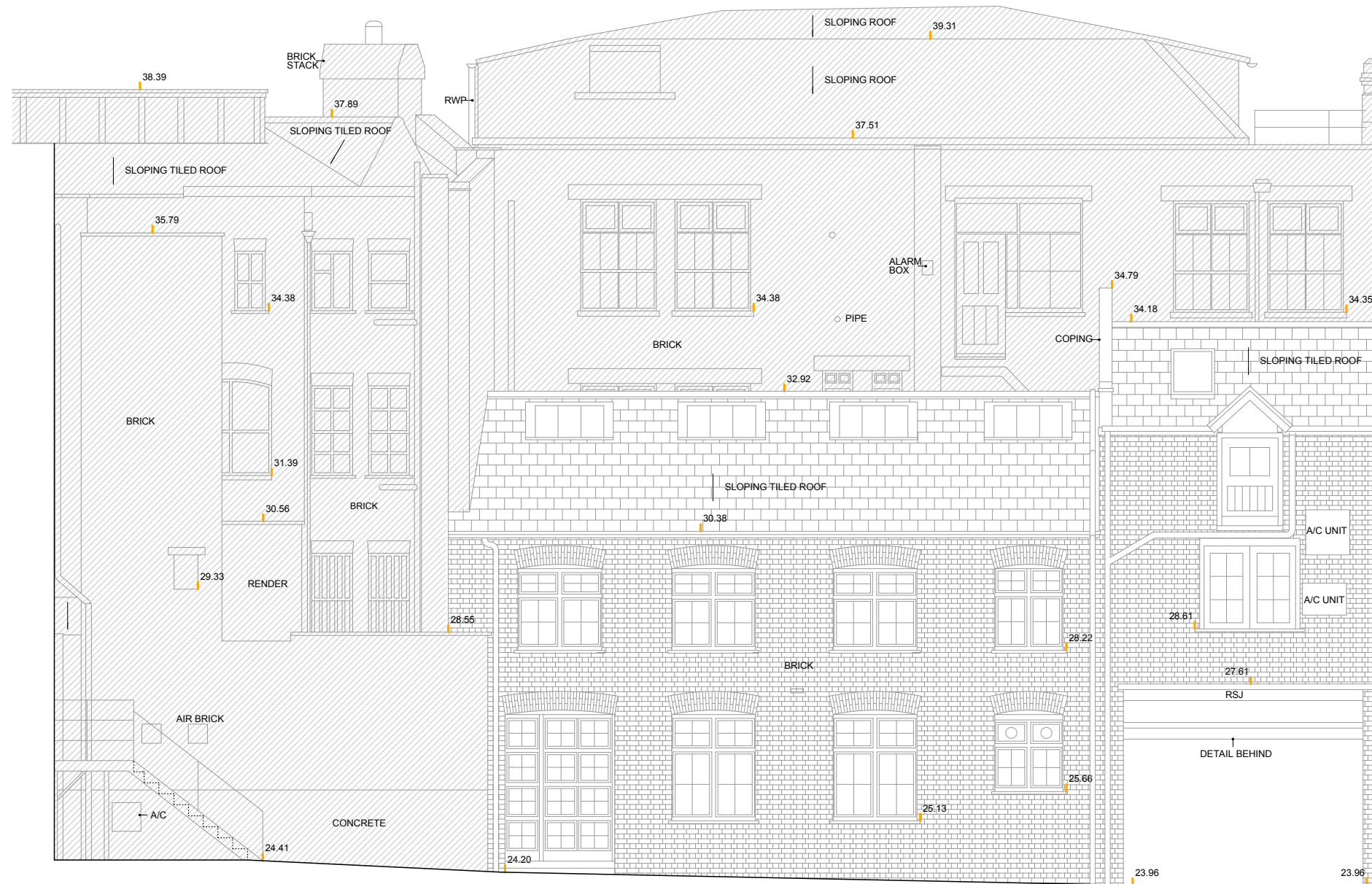
1 No1 BOOK MEWS EXISTING ELEVATION 3
