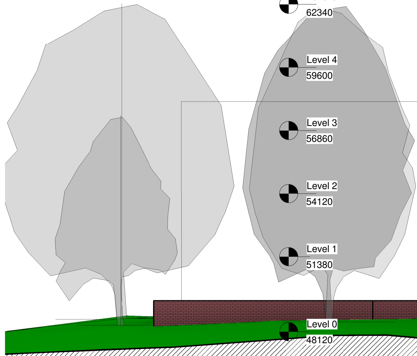
East Elevation from Primrose Hill Road - 1/100 @ A1 or 1/200 @ A3
