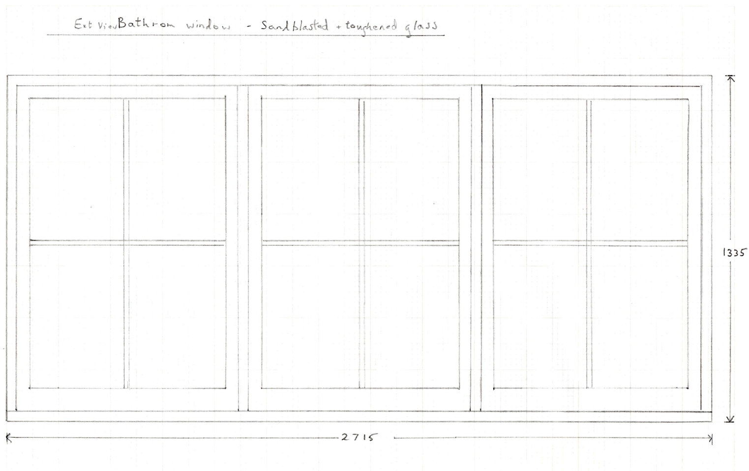
Figure 2 - side windows, bathroom (existing and proposed)
