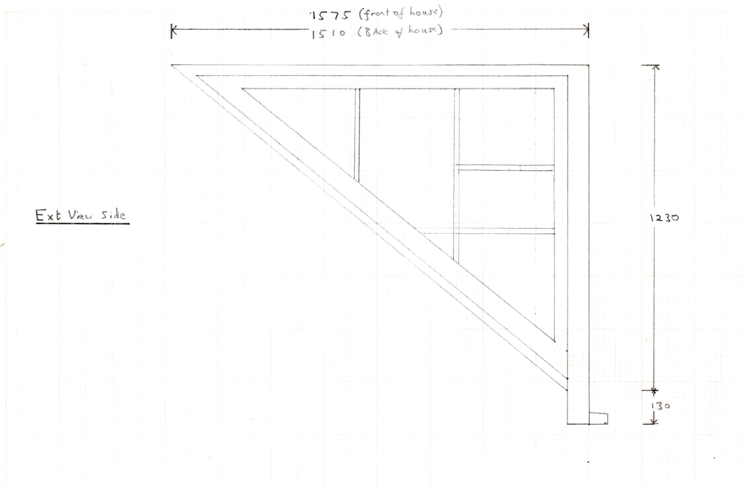
Figure 3 - side windows, dormer (existing and proposed)
