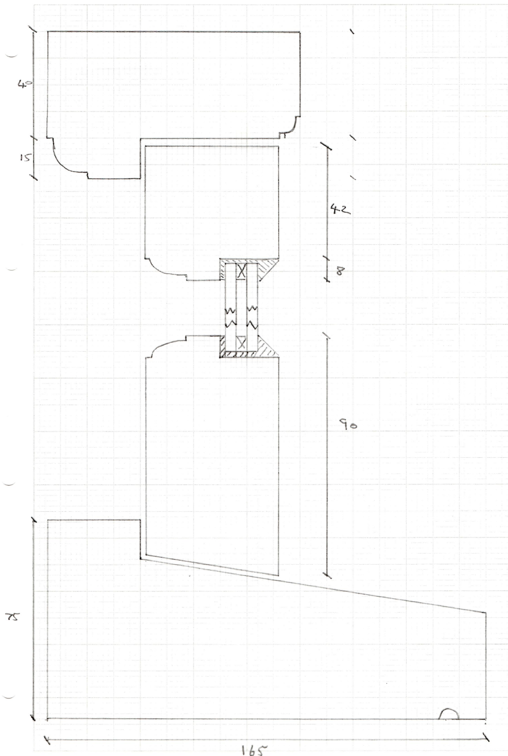
Figure 4 - detail plan view showing front and rear window frame sizing and design (proposed)
