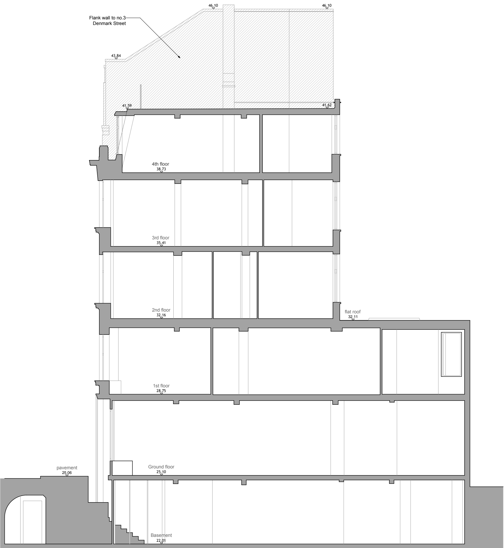
3 No4 DENMARK STREET EXISTING SECTION D-D
