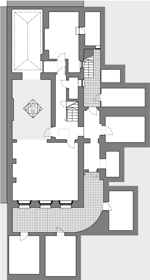
Key plan / Lower Ground Floor (1:200@A3)
