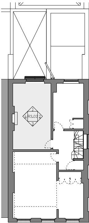
Key plan / Third Floor (1:200@A3)
