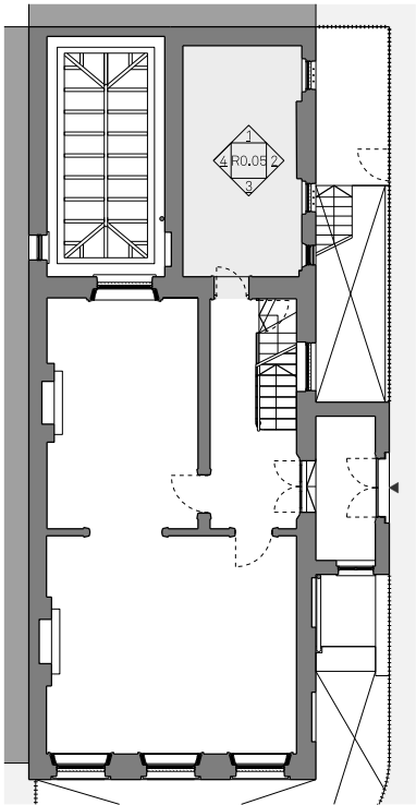
Key plan / Ground Floor (1:200@A3)
