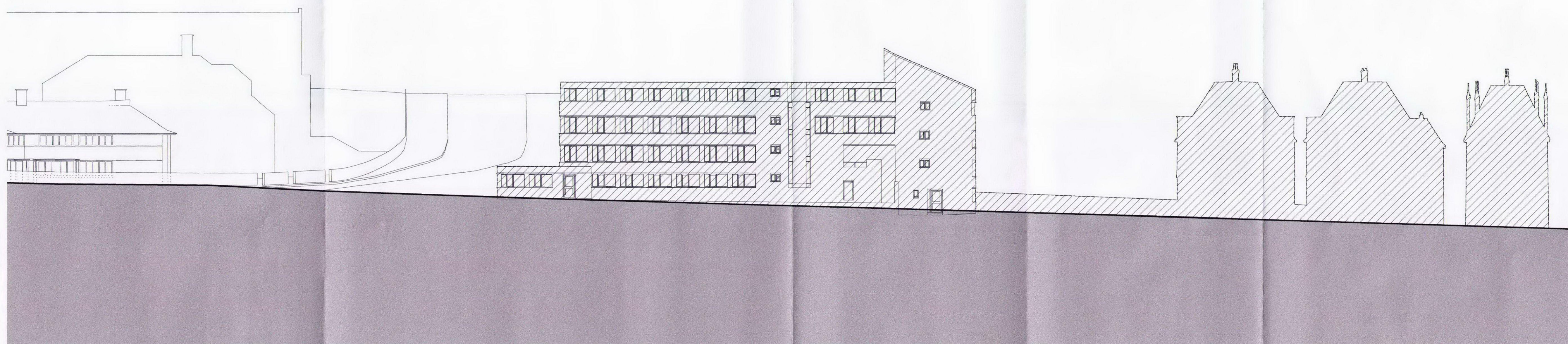
Platt's Lane NW & Finchley Road SW Elevation
