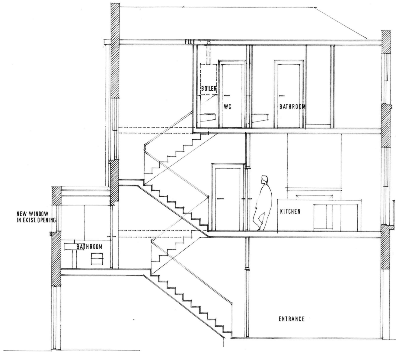
Section A-A proposed
