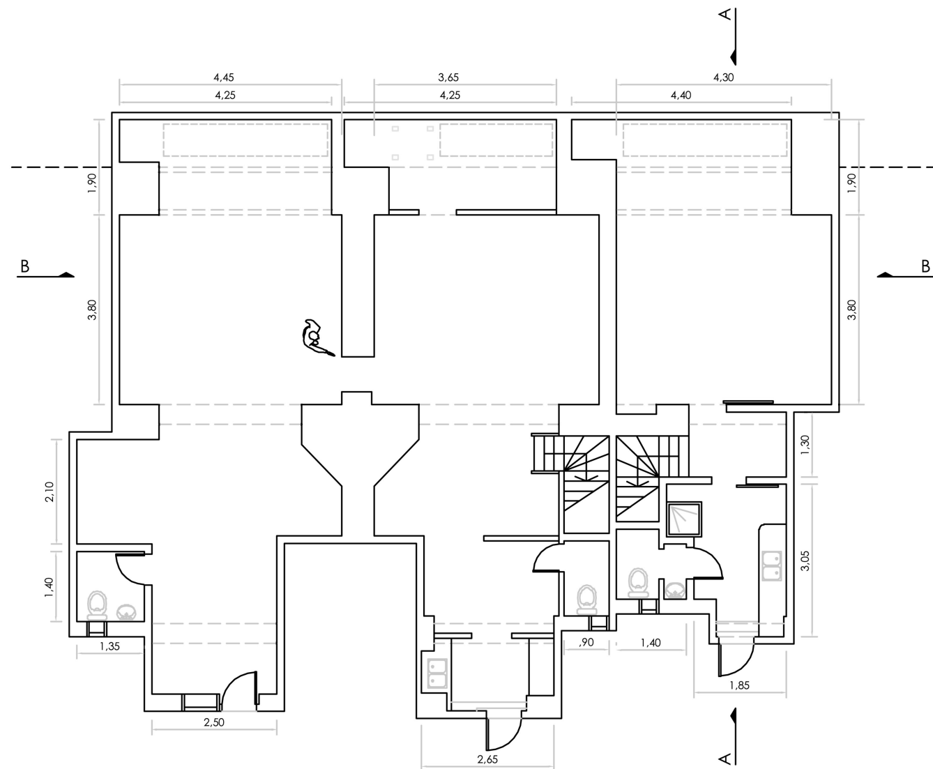
BASEMENT
