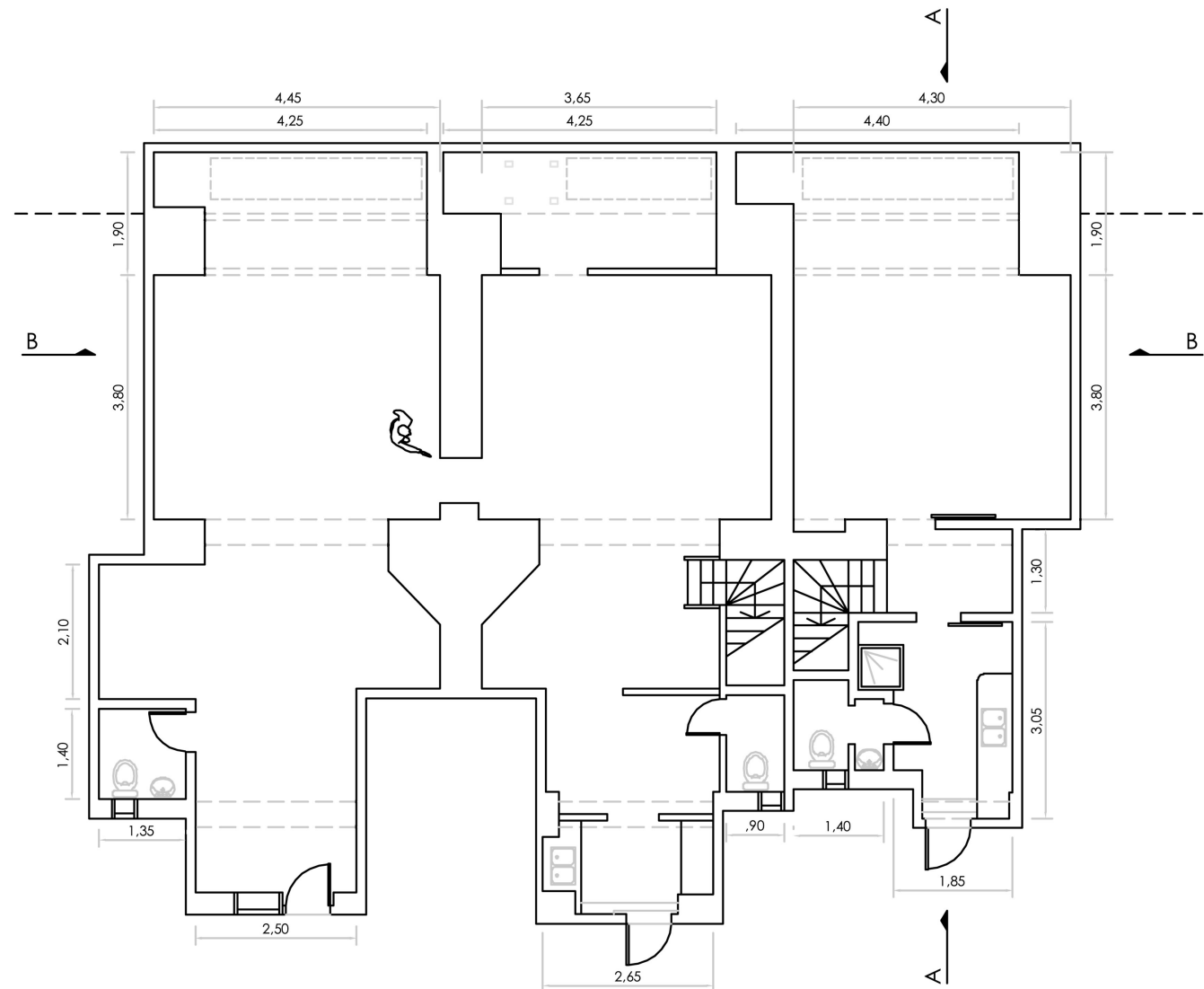
BASEMENT
