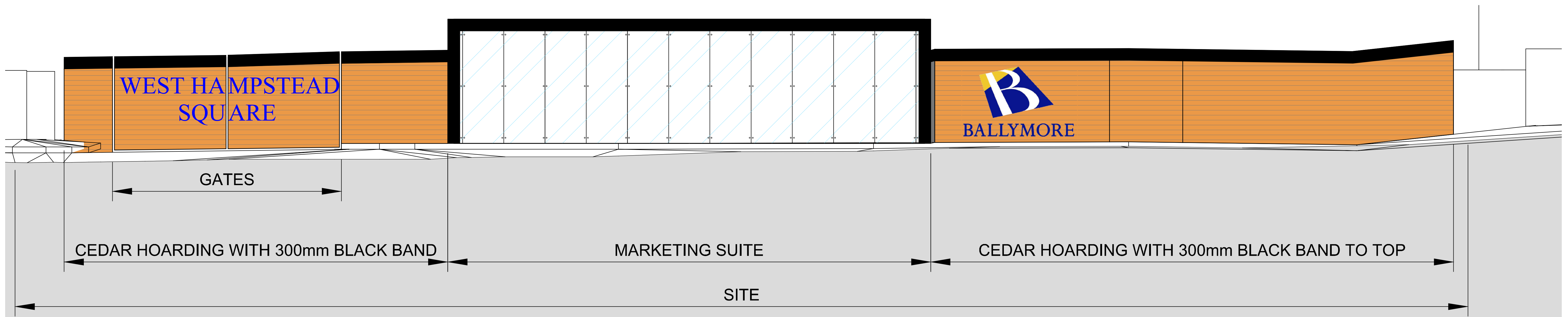
A Site Section A (Front of Marketing Suite) Scale 1:50 @ A1, 1:100 @ A3
