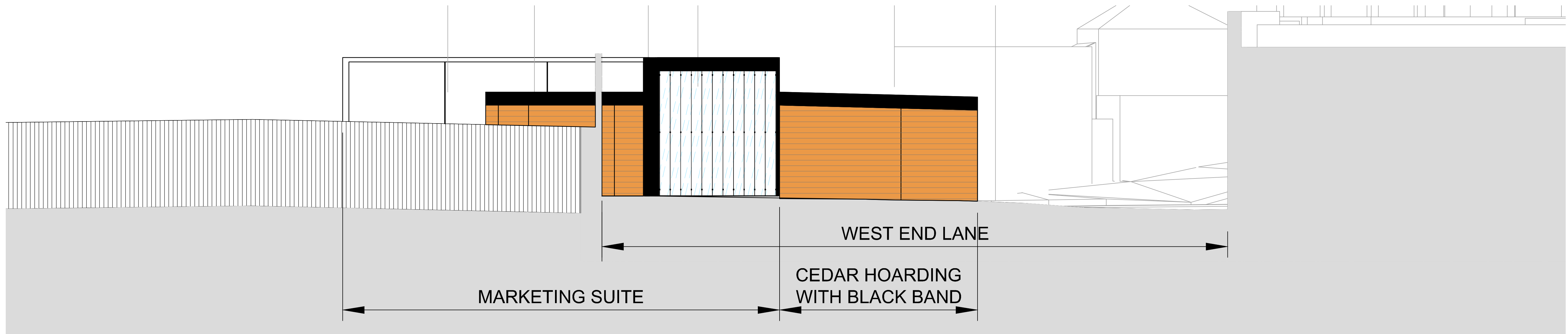
B Site Section B (Side of Marketing Suite) Scale 1:50 @ A1, 1:100 @ A3
