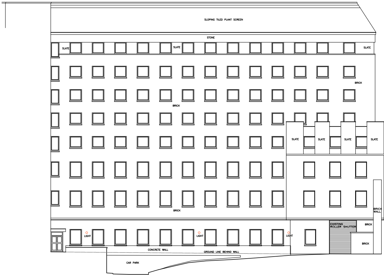
45.000m AD Car Park Elevation (2)
