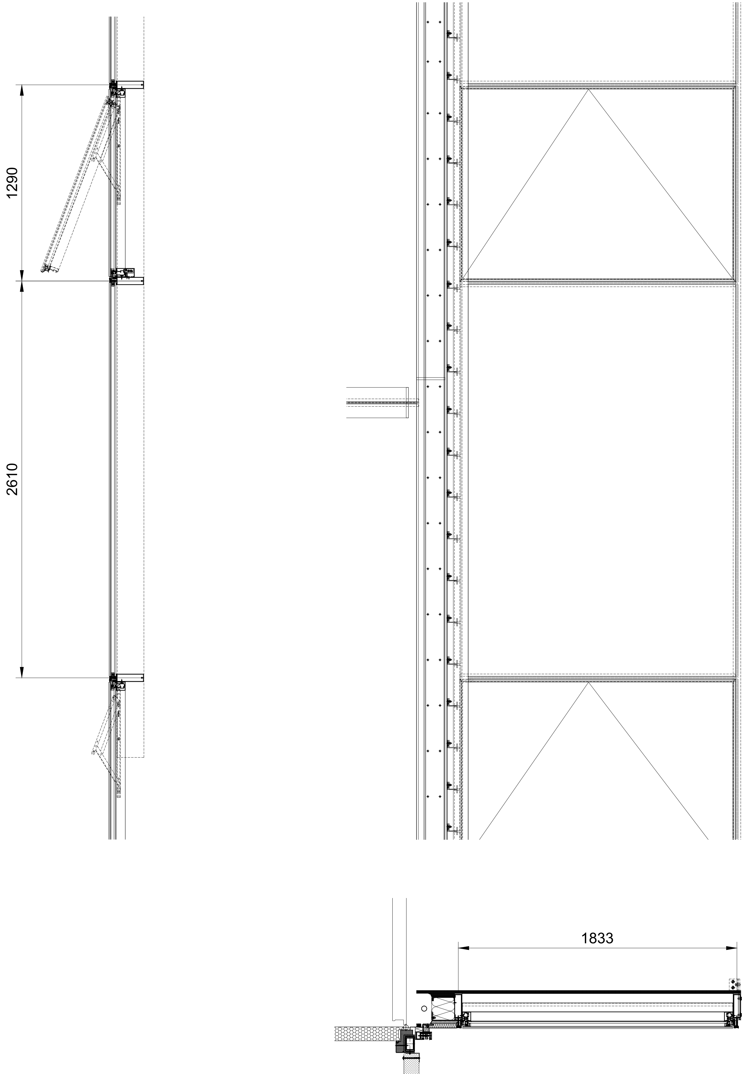
EWS-6B Scale 1:20 @A2
