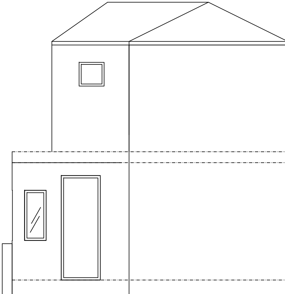
SOUTH WEST ELEVATION AS EXISTING
