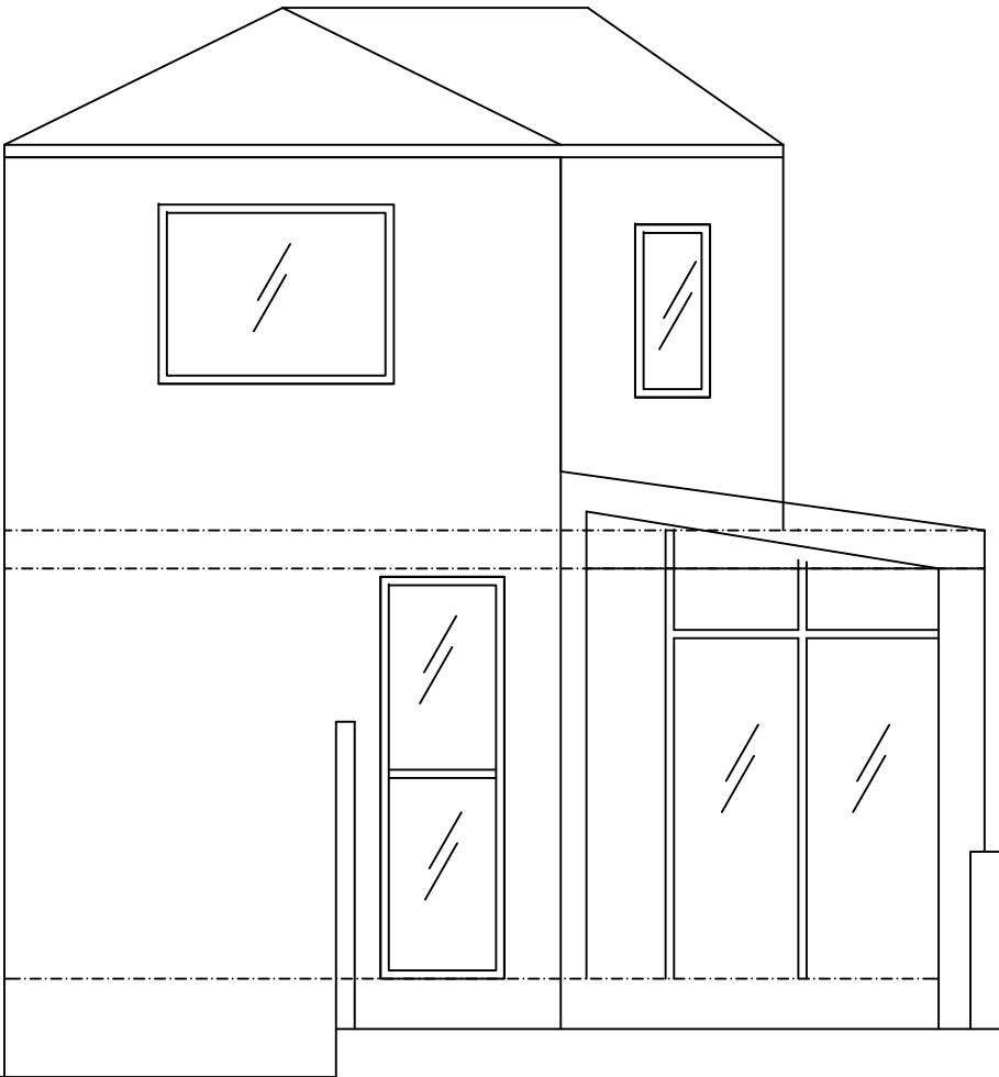
NORTH EAST ELEVATION AS EXISTING
