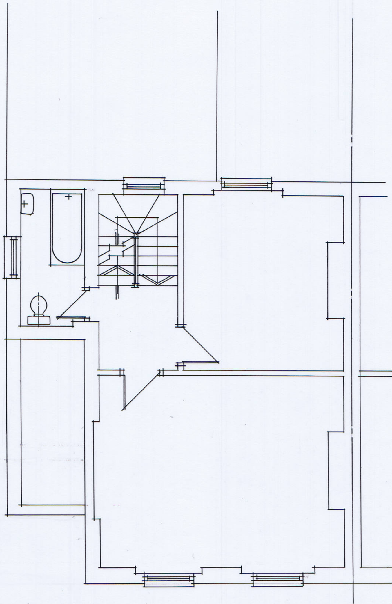
EXISTING FIRST FLOOR PLAN
