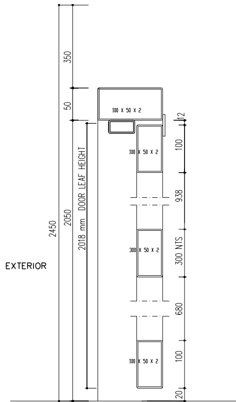
HEIGHT SECTION THRO' GRILLE GATE
