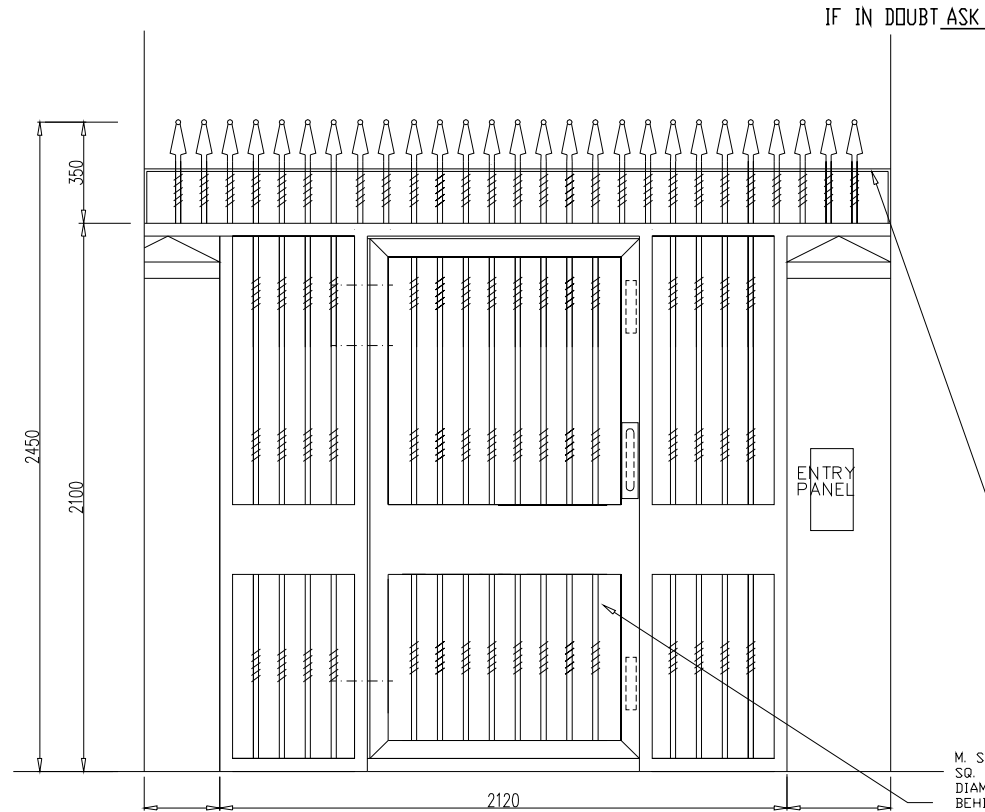
ELEVATION OF TYPICAL GRILLE GATE HLOI DOOR OPENING IN AWAY FROM VIEWER
