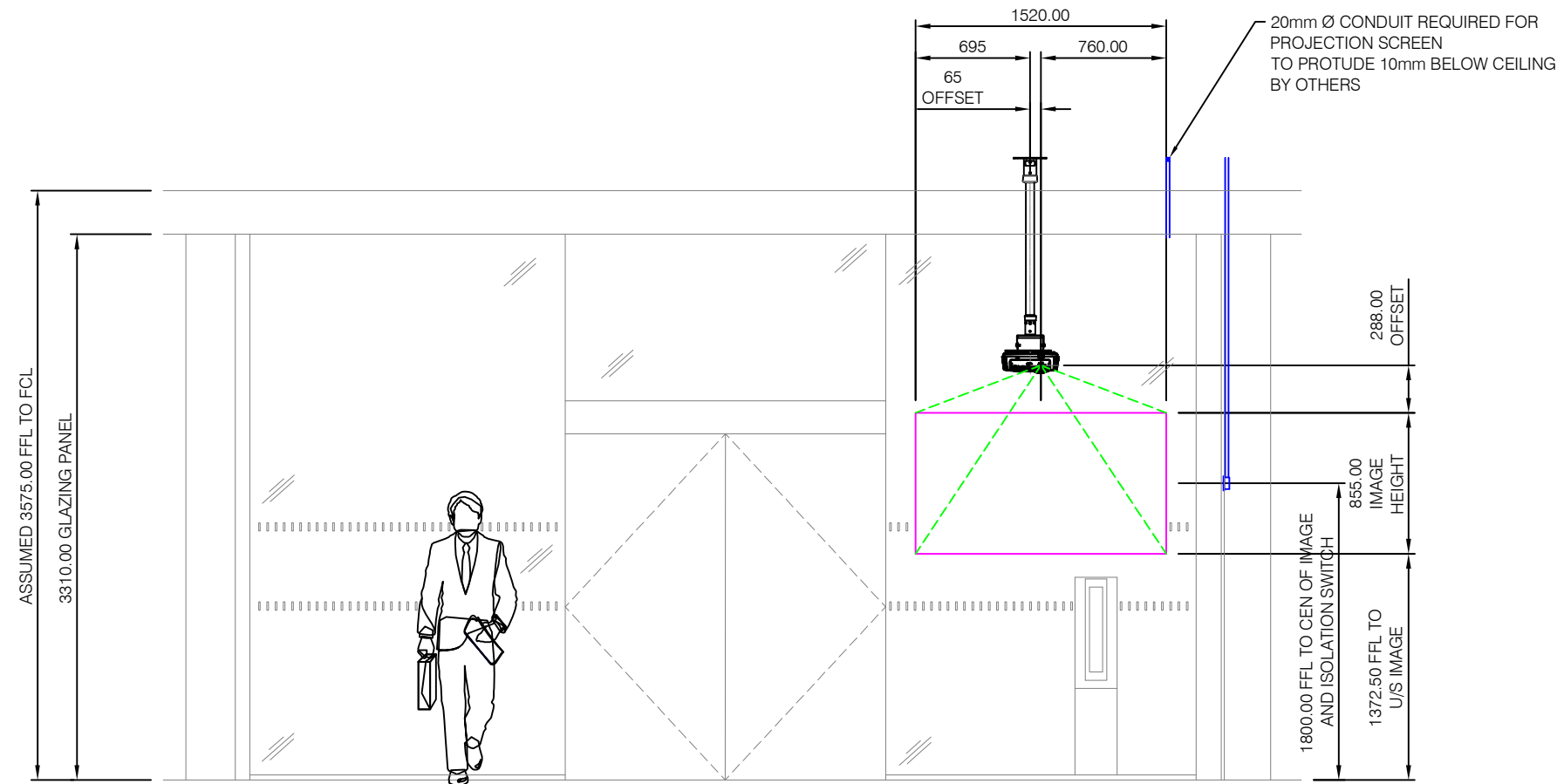
ELEVATION ON A - A
