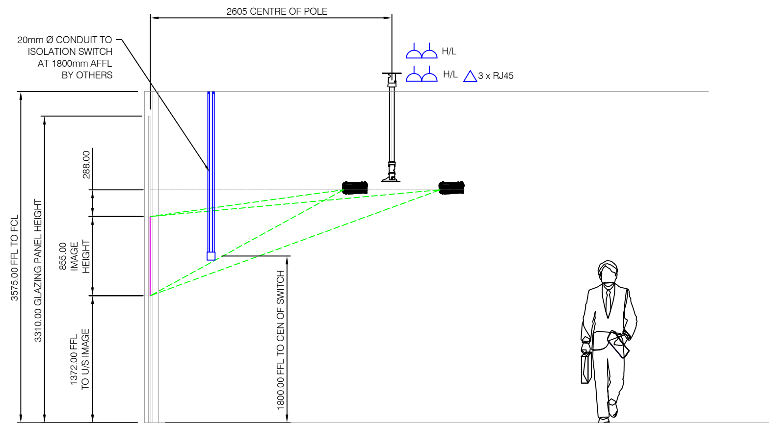
ELEVATION ON B - B
