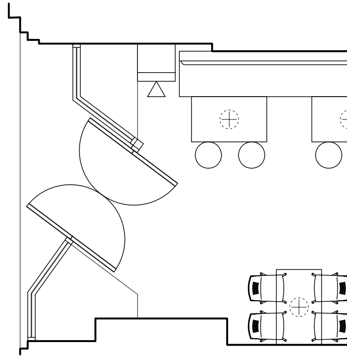
EXISTING PLAN
