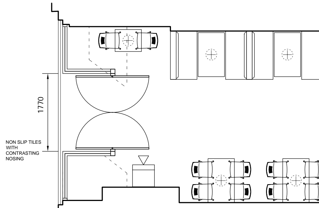
PROPOSED PLAN
