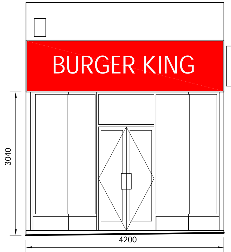
EXISTING ELEVATION
