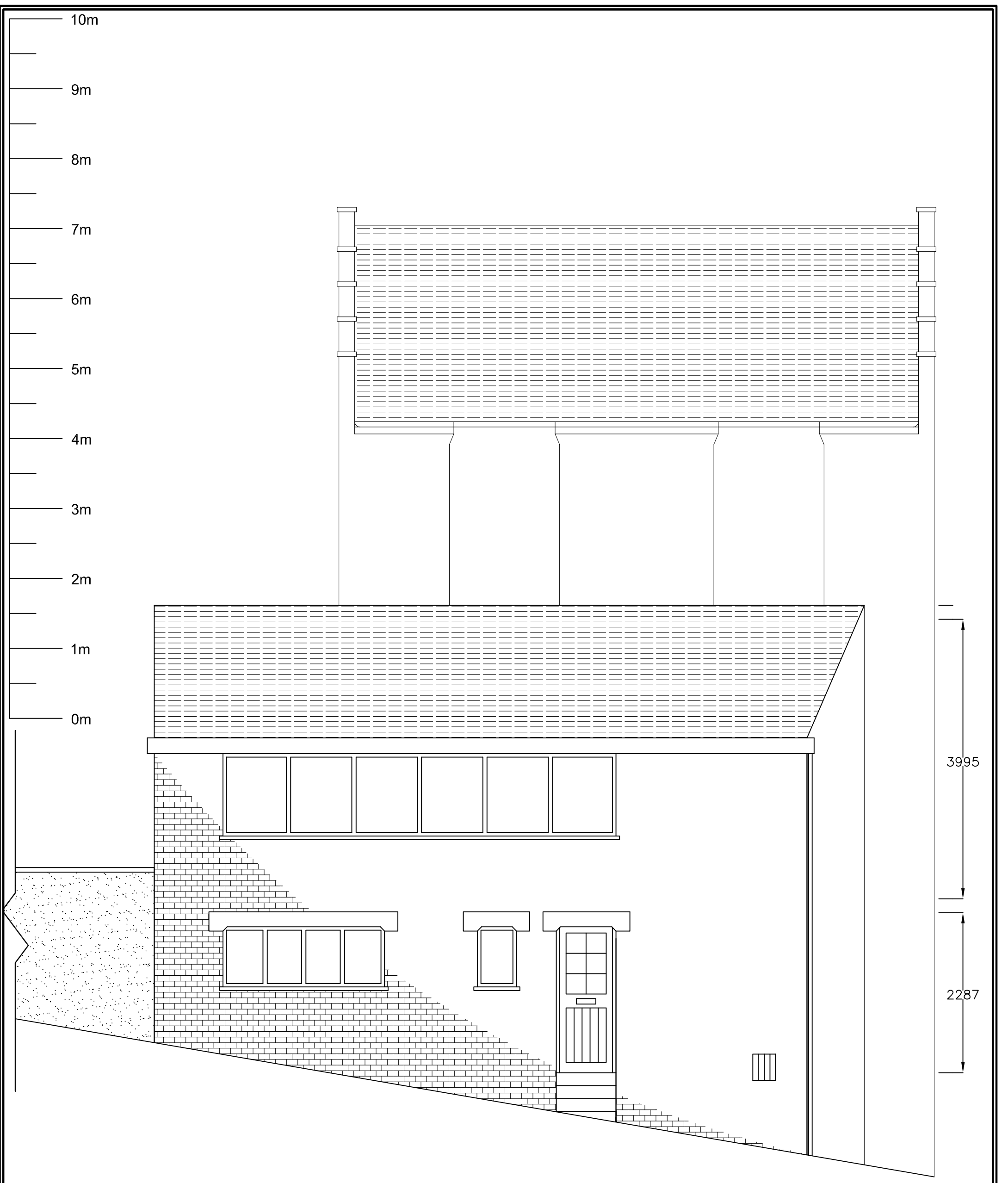
FRONT ELEVATION EXISTING
