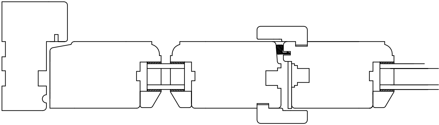
MUMFORD & WOOD LTD. CONSERVATION FRENCH DOORSET JAMB DWG.No. FDJ
