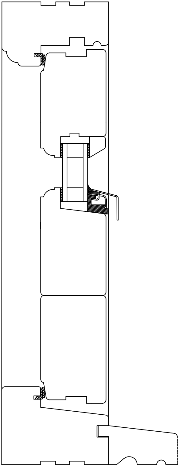
MUMFORD & WOOD LTD. CONSERVATION FRENCH DOORSET HEAD/CILL DWG.No. FDHC
