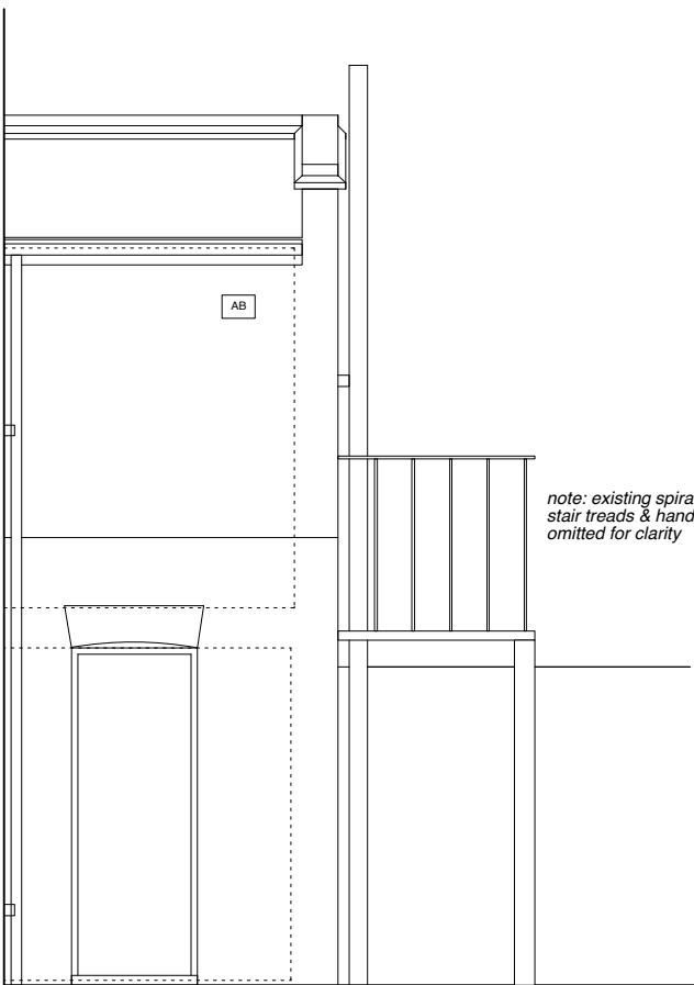
BACK EXTENSION SIDE ELEVATION
