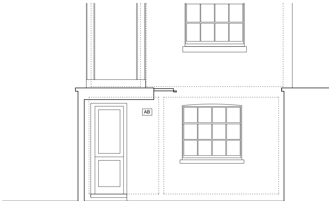
EXISTING FRONT AREA ARRANGEMENT (RAILINGS/BALUSTRADING OMITTED FOR CLARITY)
