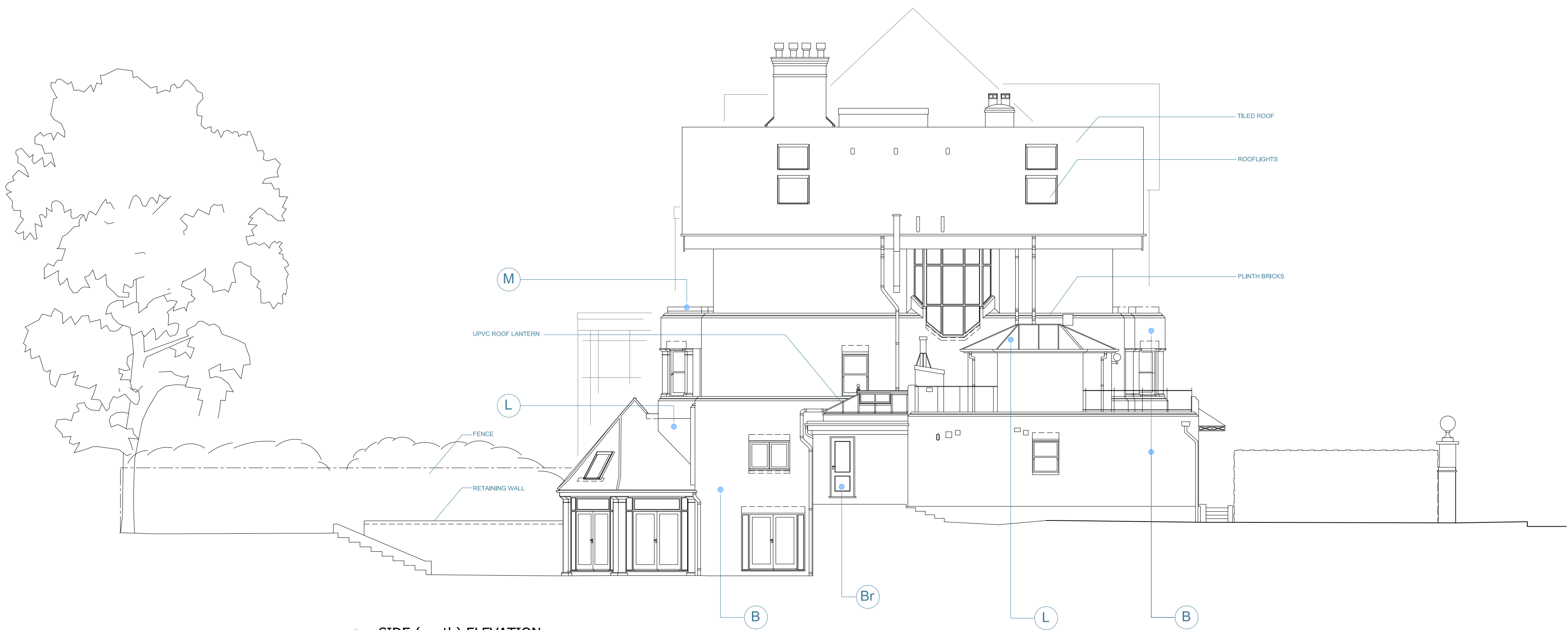
3 SIDE (south) ELEVATION
