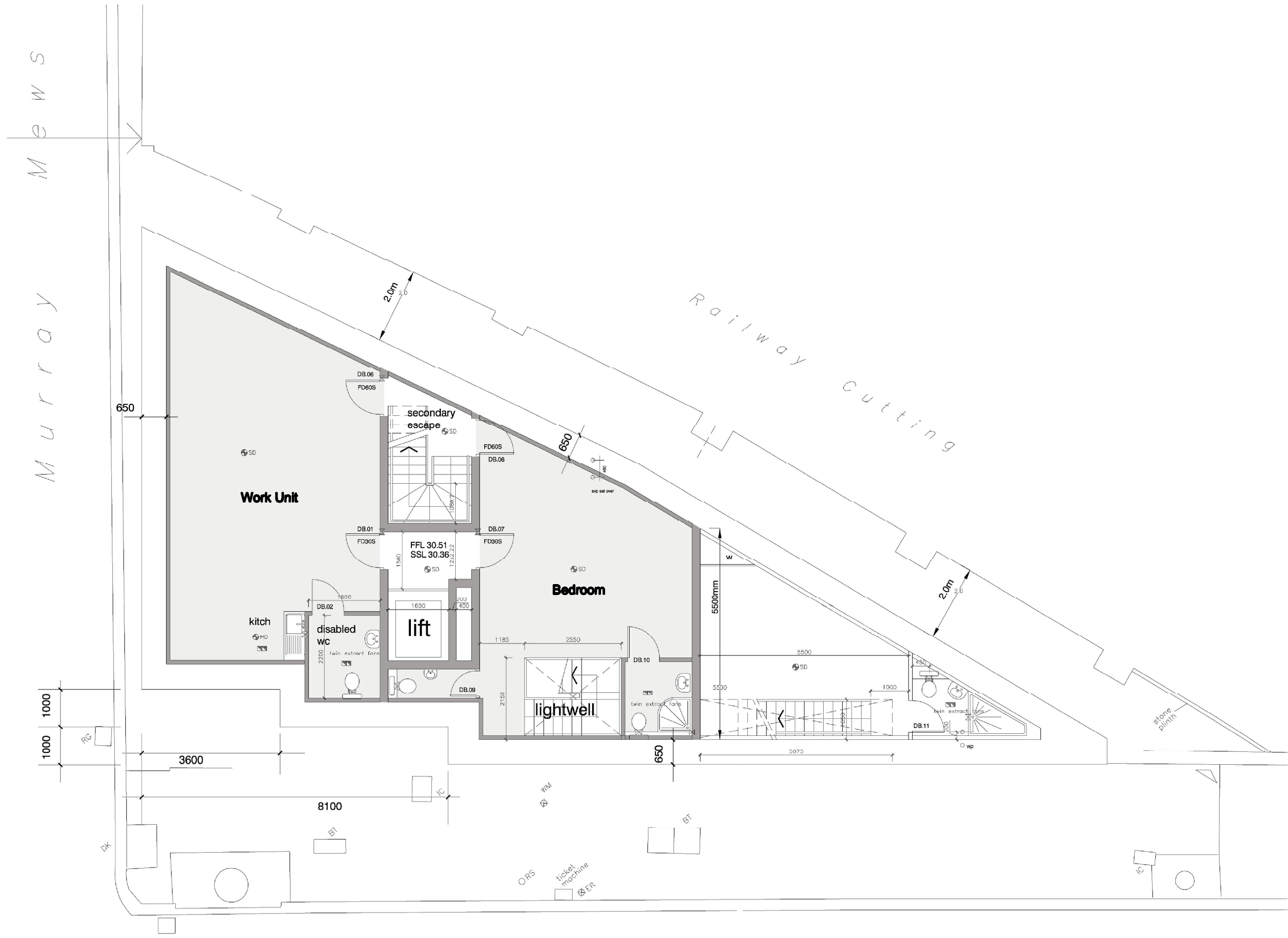
1 PROPOSED BASEMENT FLOOR PLAN Scale 1:100 @A3
