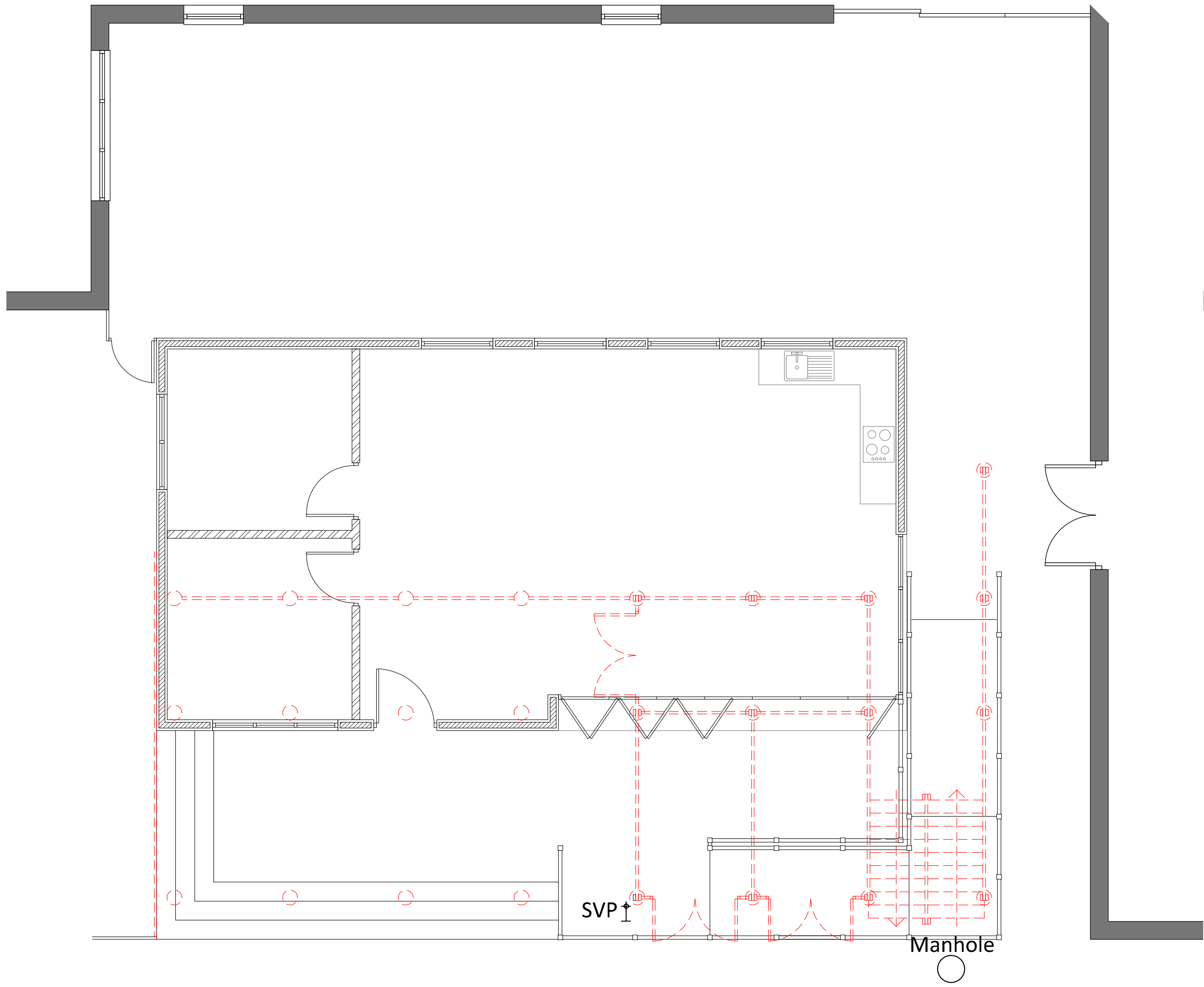
Demolition Plan - Ground Floor
