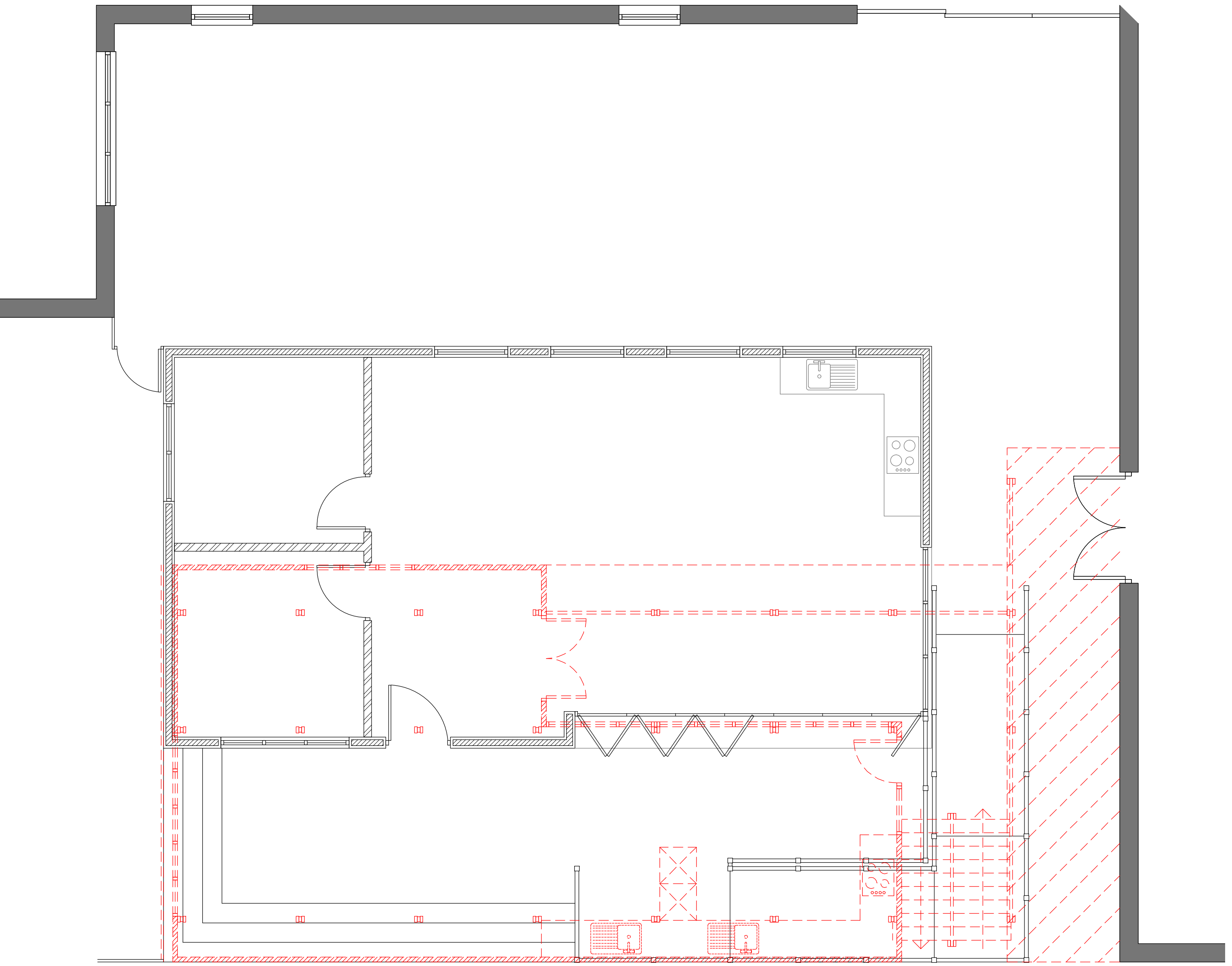
Demolition Plan - First Floor
