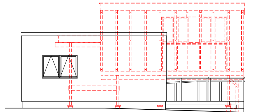
North East Elevation with Demolition
