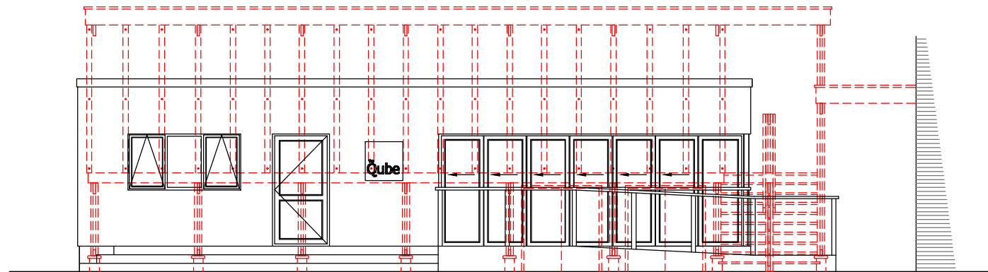
North West Elevation with Demolition
