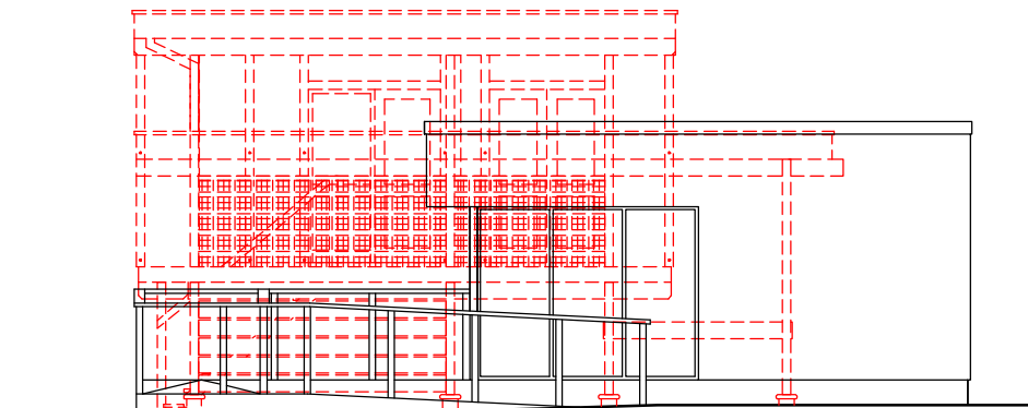
South West Elevation with Demolition
