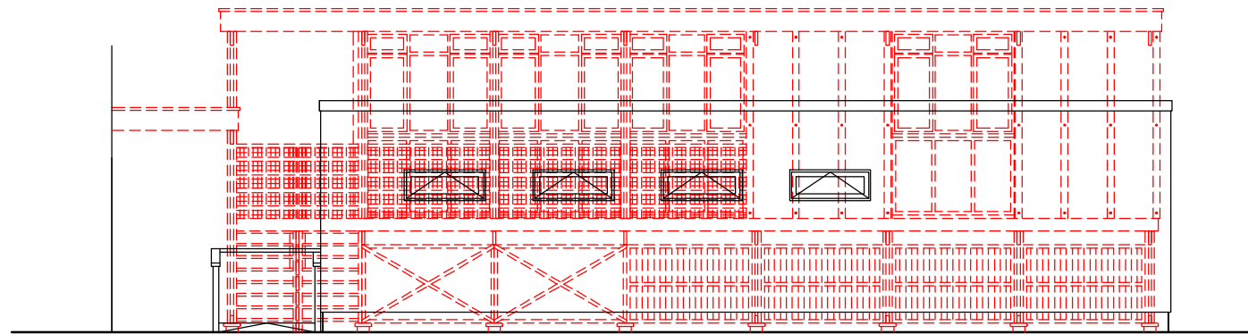
South East Elevation with Demolition
