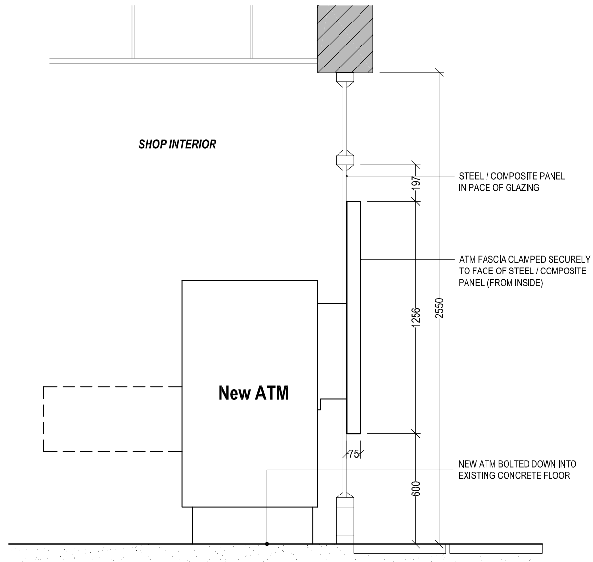
TYPICAL SECTION THROUGH WINDOW INSTALLATION Scale 1:25
