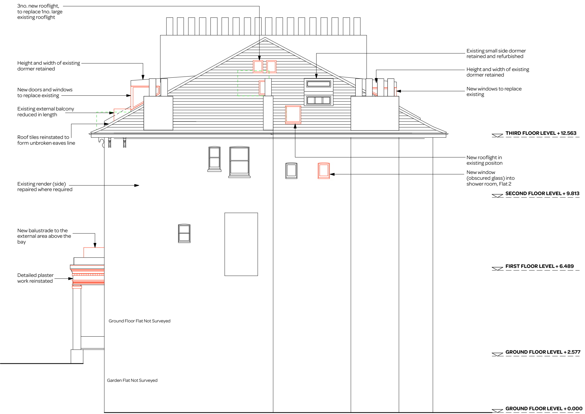
Side Elevation (Part Surveyed)
