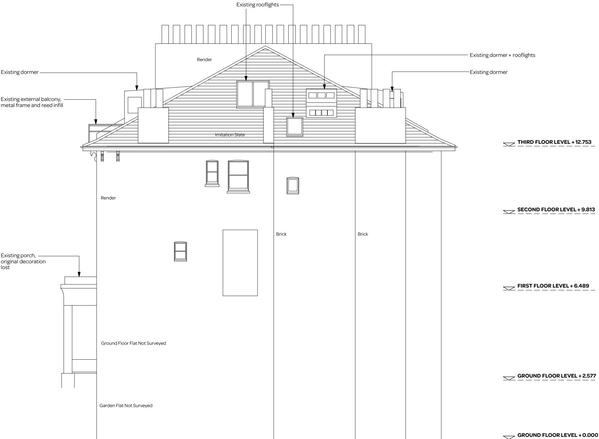
Side Elevation (Part Surveyed)
