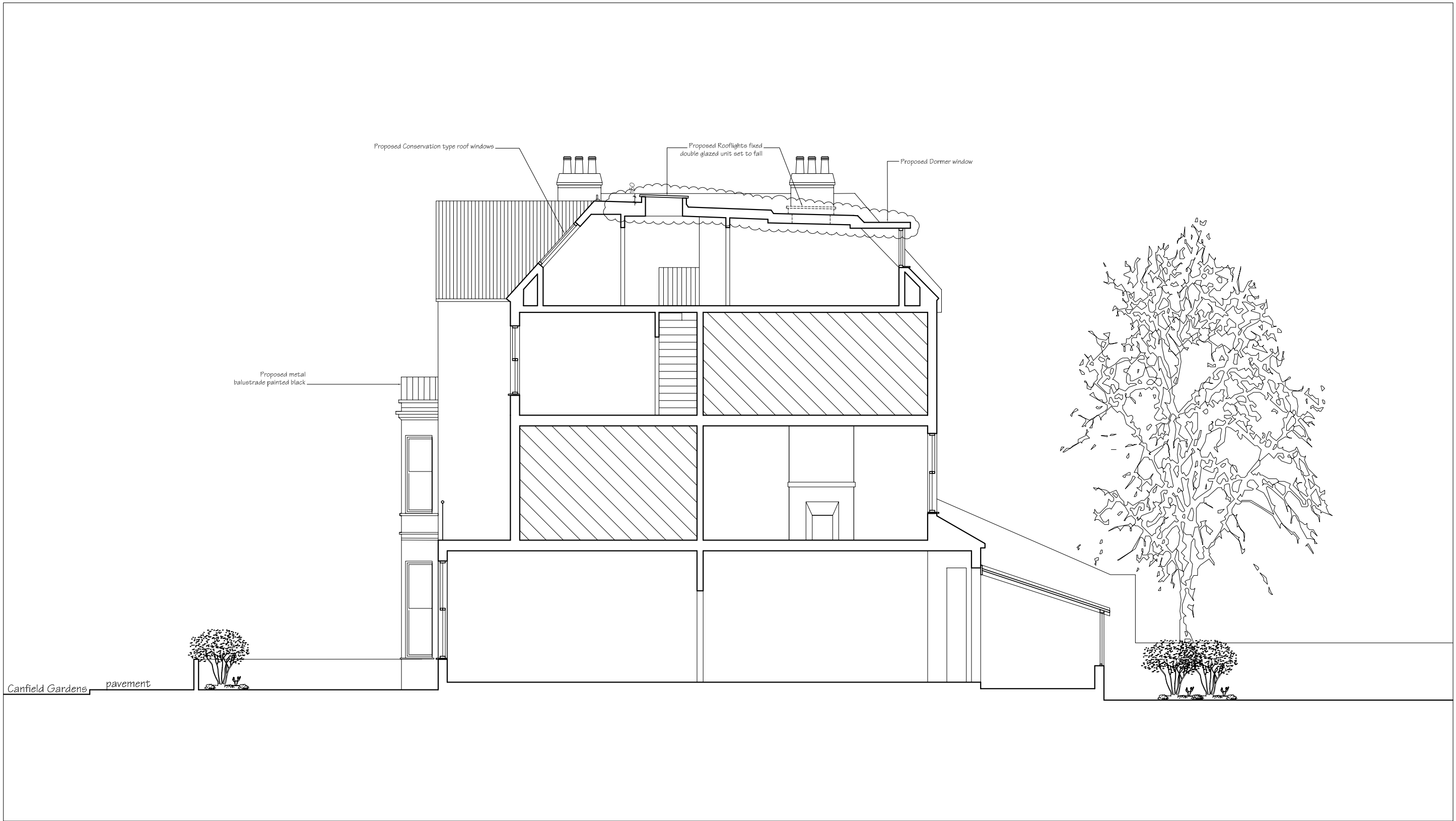
Cross Section A-A as Proposed
