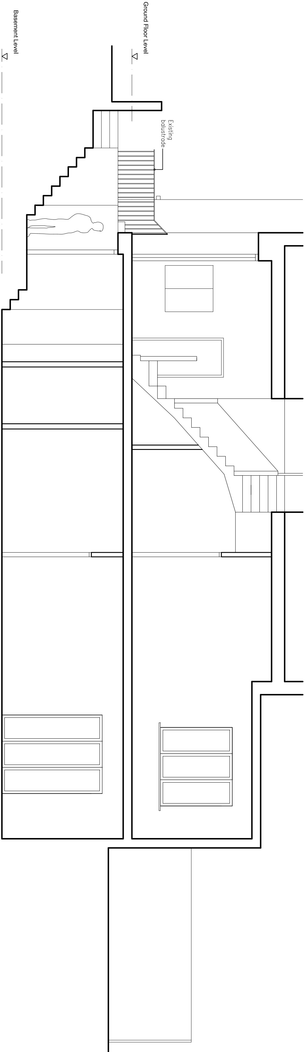
Proposed Section BB
