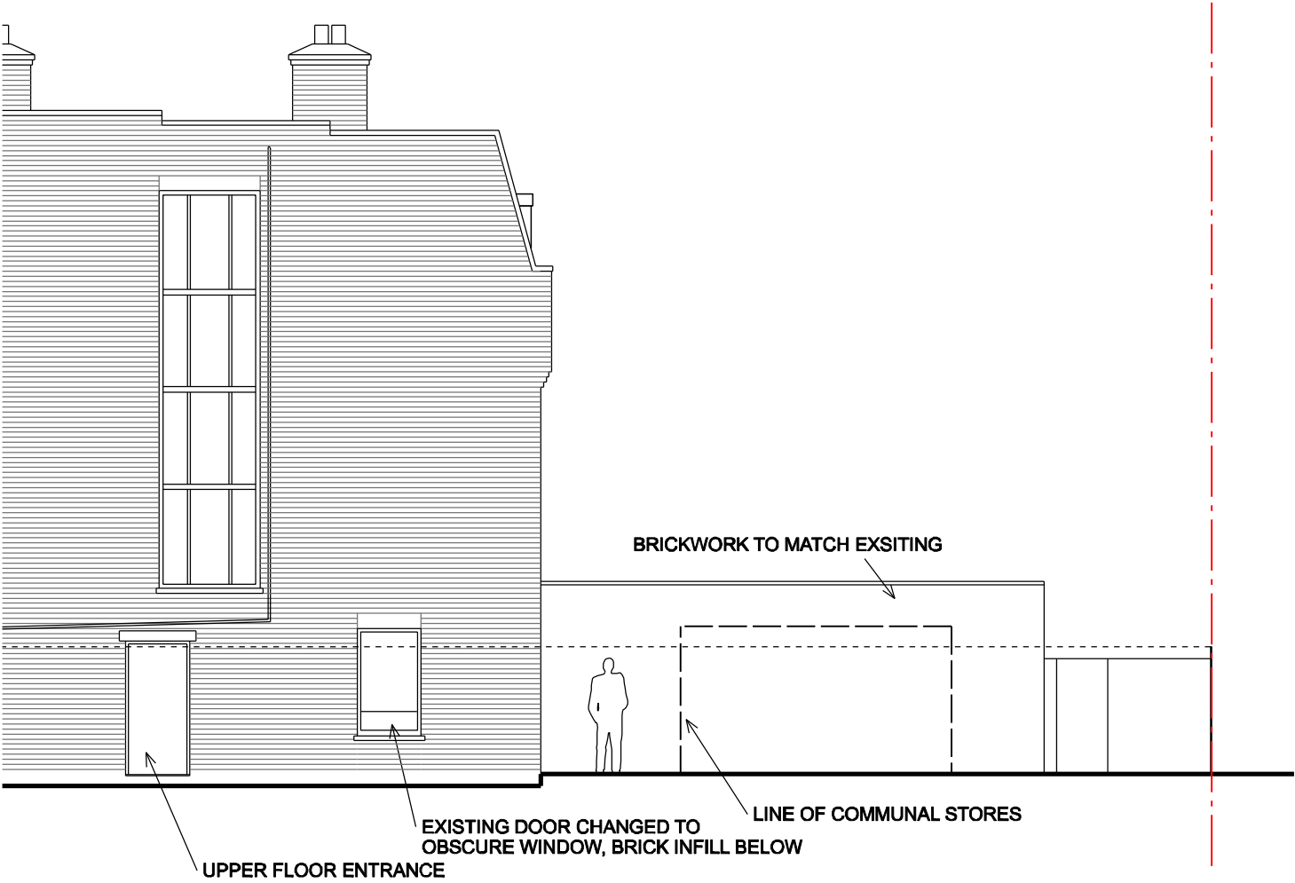
SIDE ELEVATION
