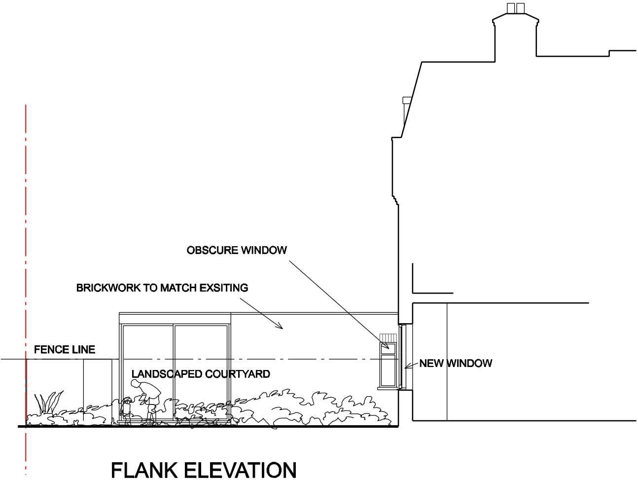
SIDE ELEVATION
