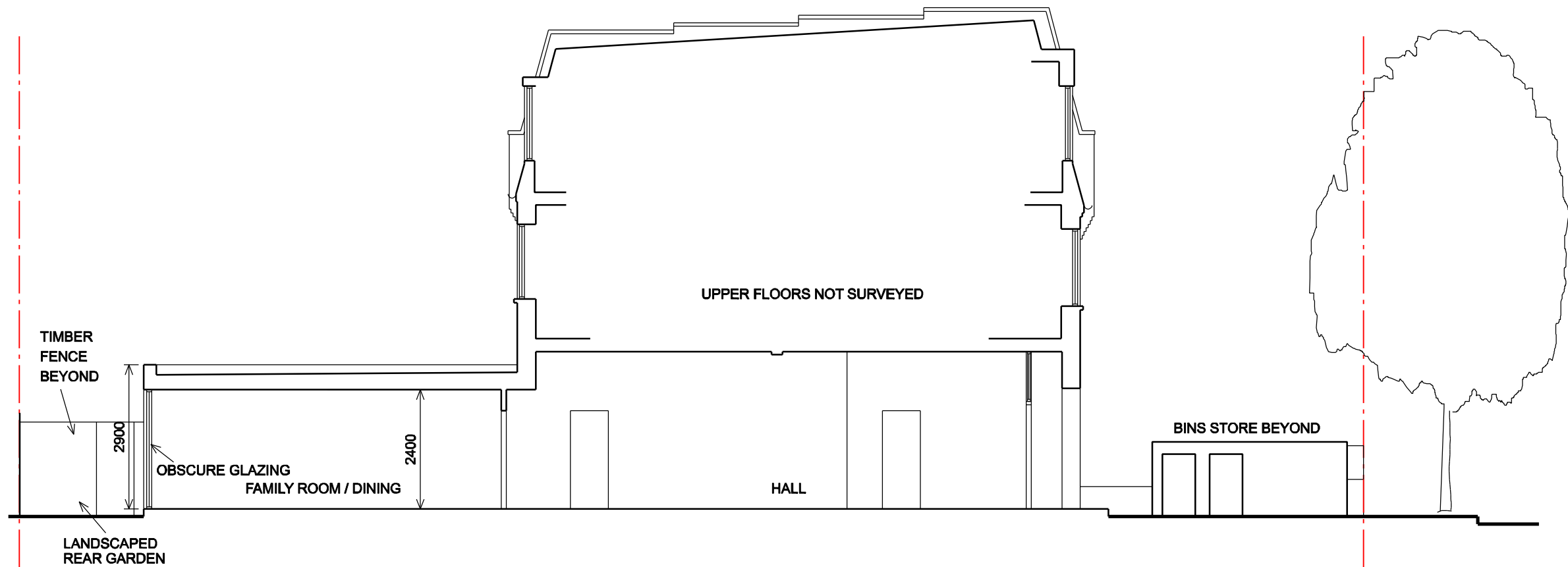
TYPICAL SECTION
