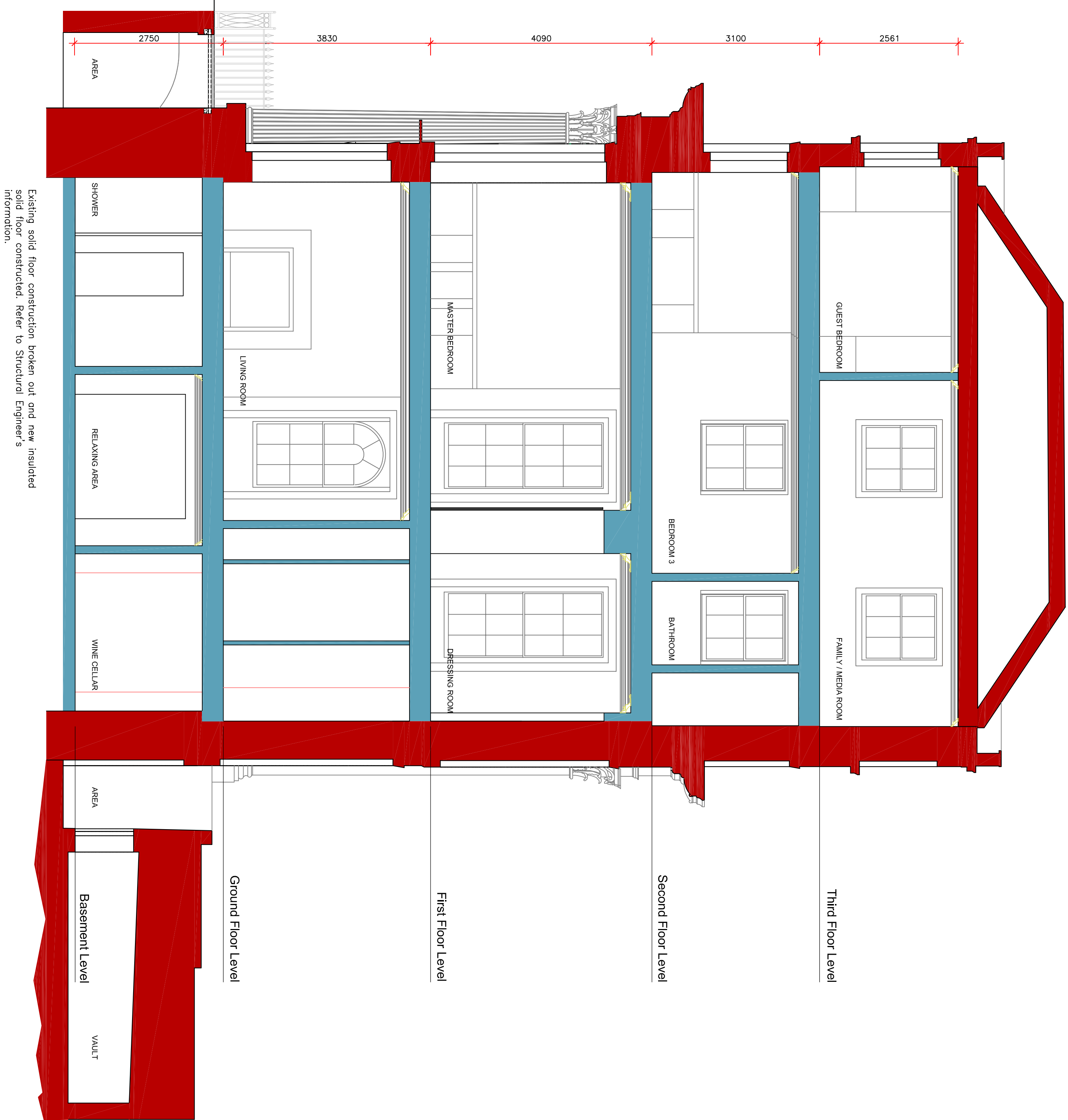
PROPOSED SECTION AA
