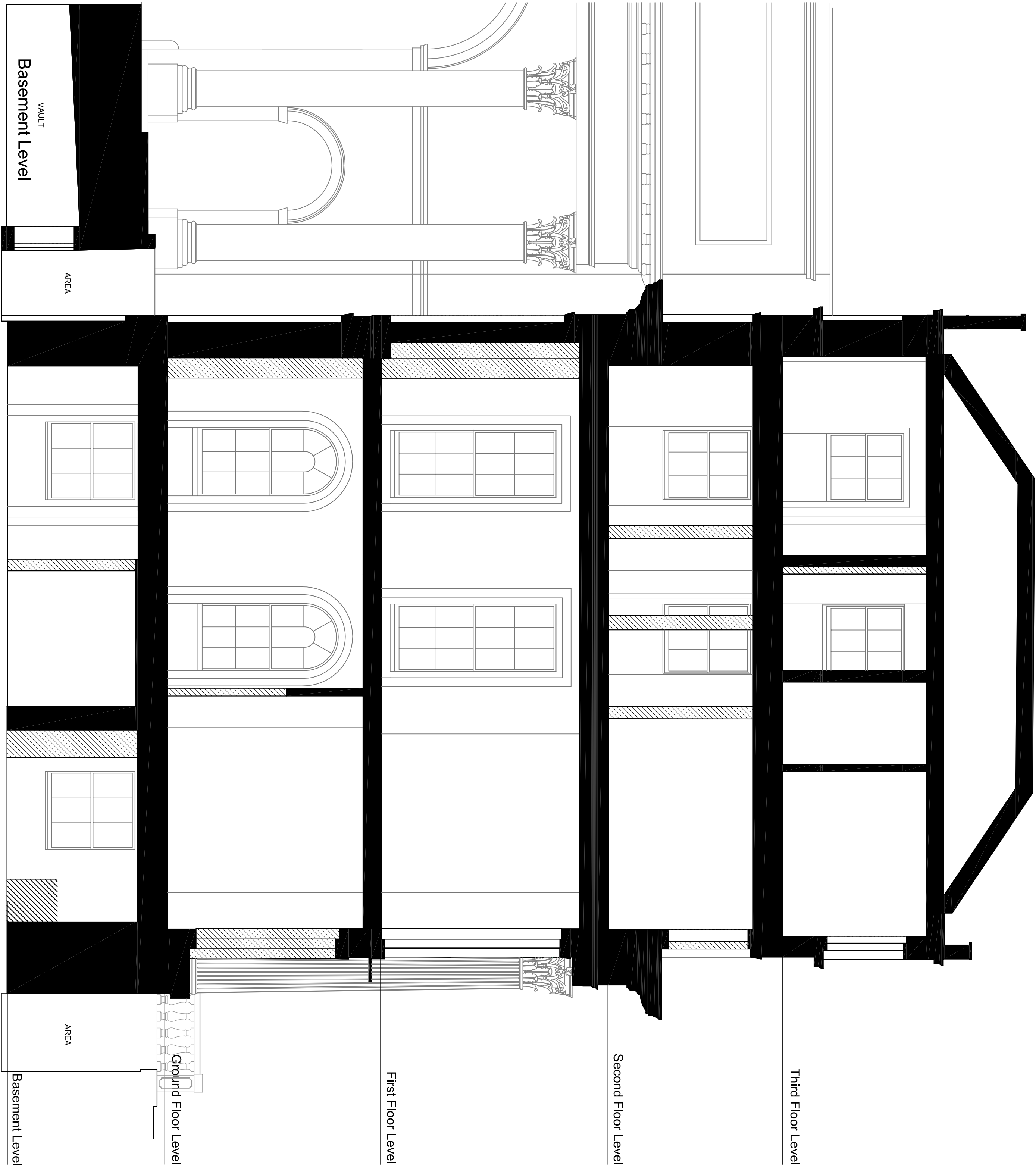
EXISTING SECTION CC
