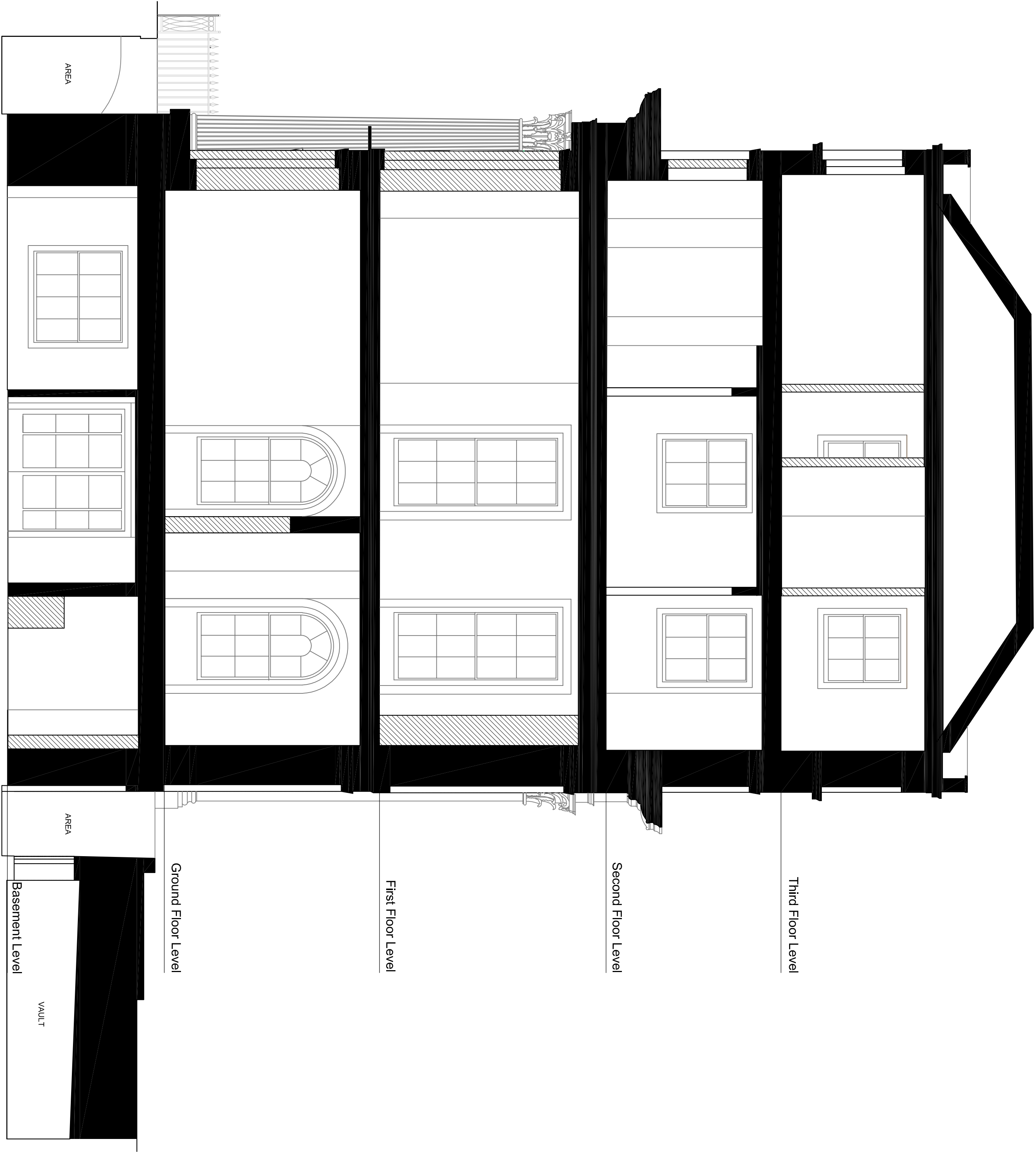
EXISTING SECTION AA
