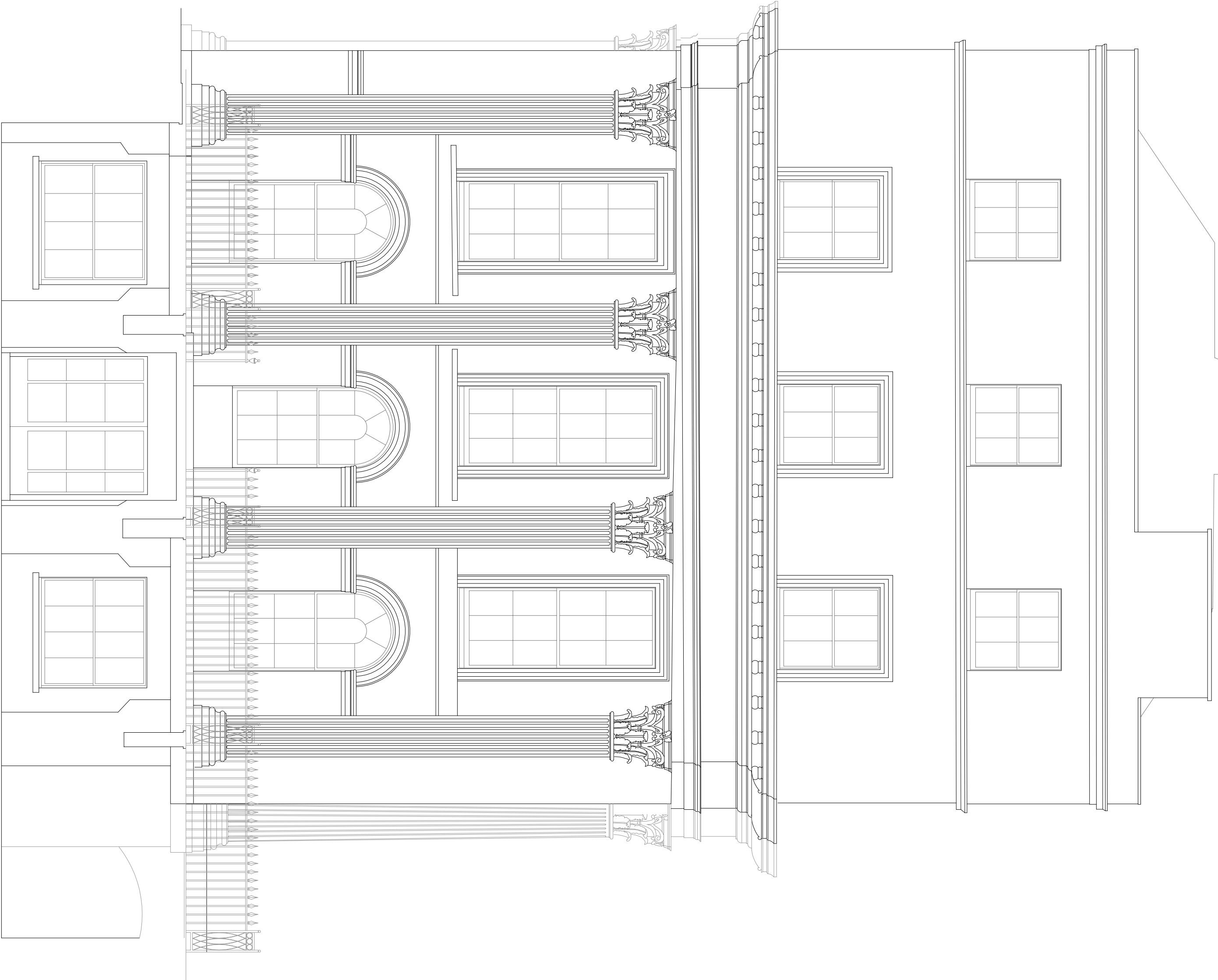
EXISTING ELEVATION 2 - NORTH
